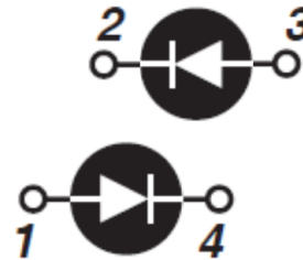
Figure 2 • Anti-parallel MSC2X30SDA120J
