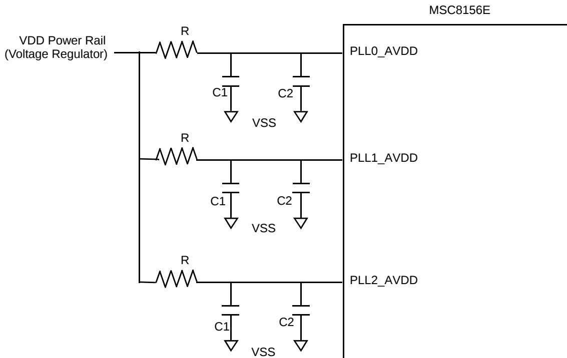
Figure 37. PLL Supplies
