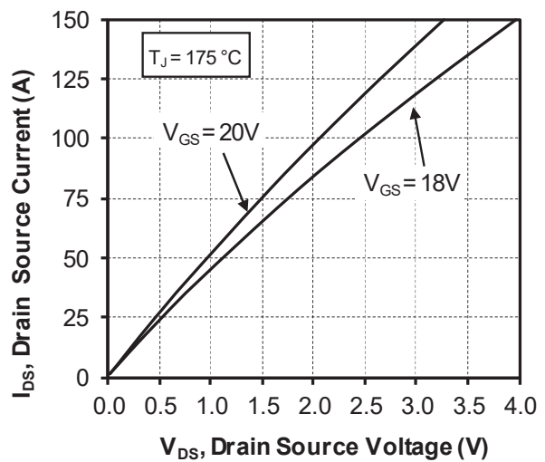
Figure 1-17. Output Characteristics, T_J = 175\text{ }^\circ\text{C}
