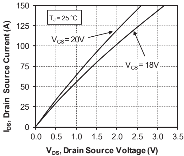
Figure 1-16. Output Characteristics, T_J = 25\text{ }^\circ\text{C}
