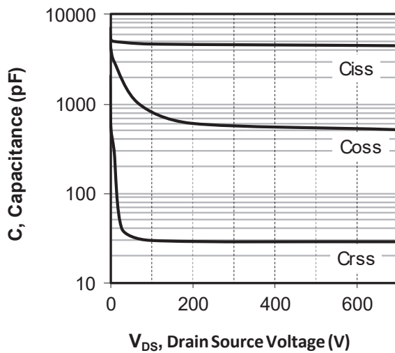
Figure 1-20. Capacitance vs. Drain Source Voltage
