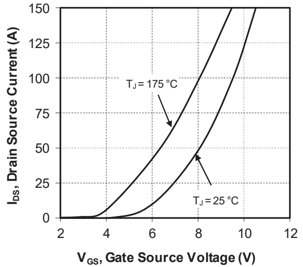
Figure 1-19. Transfer Characteristics
