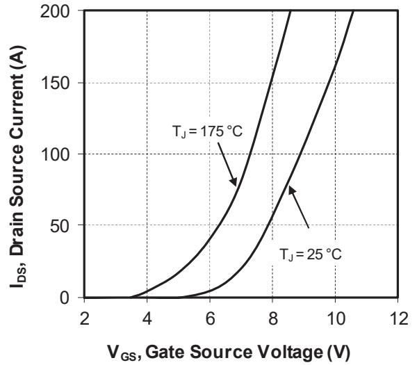
Figure 1-5. Transfer Characteristics
