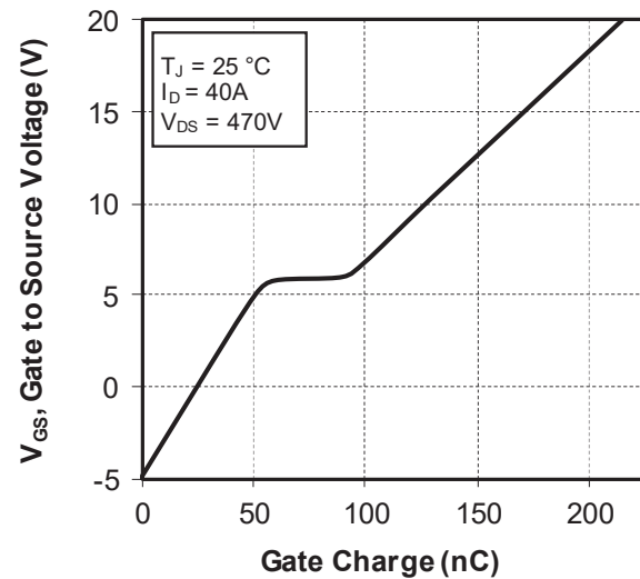
Figure 1-21. Gate Charge vs. Gate Source Voltage
