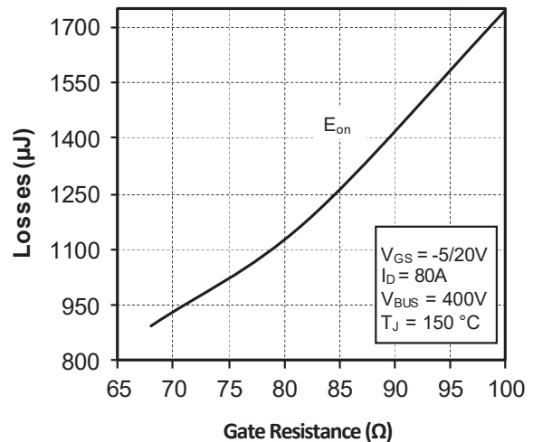
Figure 1-27. Turn On Energy vs. Rg
