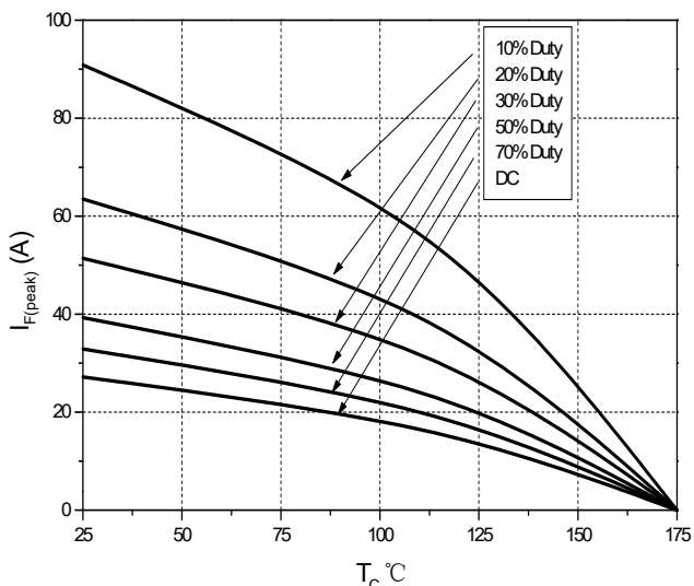
Figure 7. Current Derating
