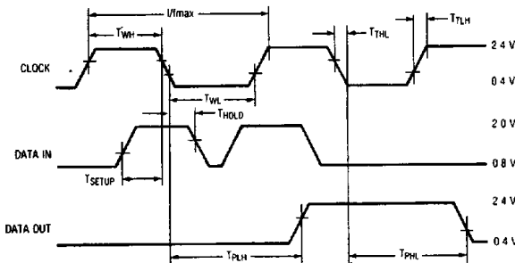
FIGURE 1. TIMING CHARACTERISTICS
