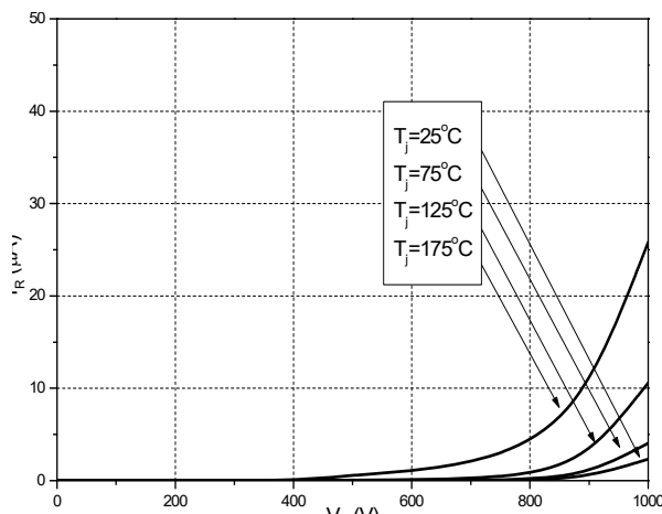
Figure 2. Reverse Characteristics
