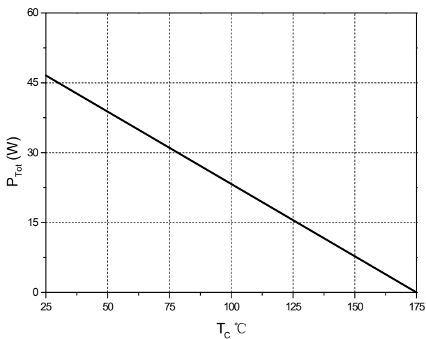
Figure 6. Power Derating
