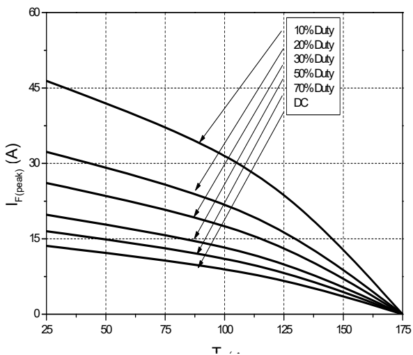
Figure 7. Current Derating
