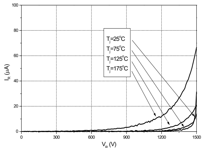
Figure 2. Reverse Characteristics
