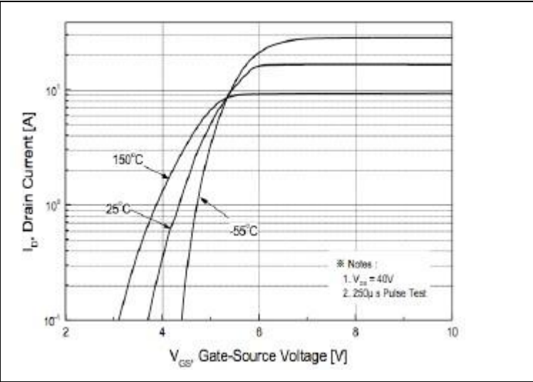
FIG.2-TRANSFER CHARACTERISTICS
