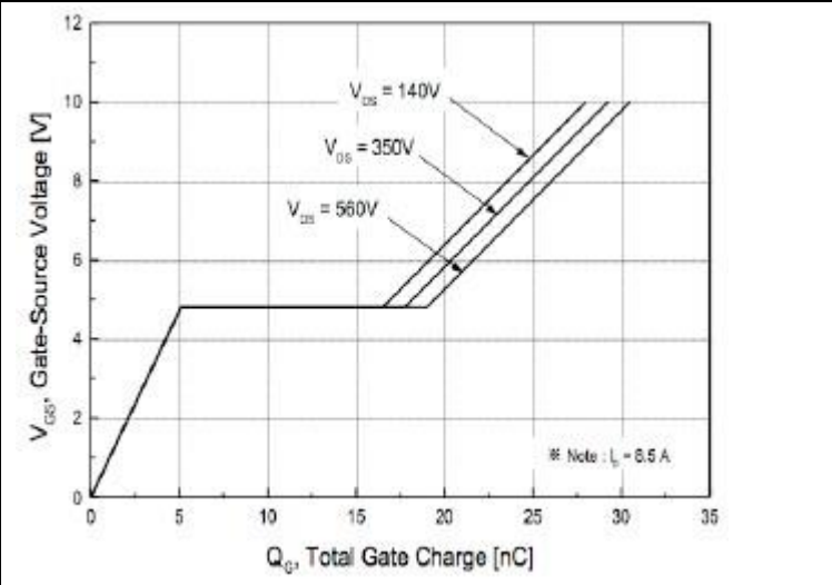
FIG.6-GATE CHARGE CHARACTERISTICS
