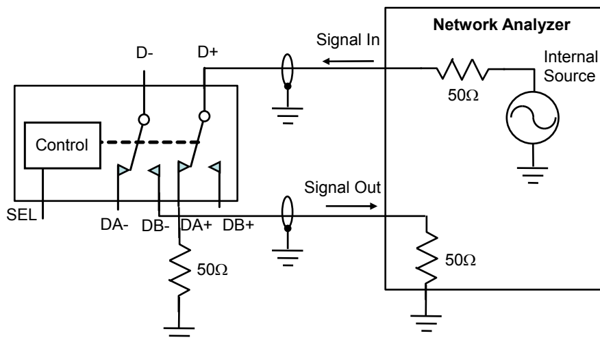
Figure 8. Channel Crosstalk
