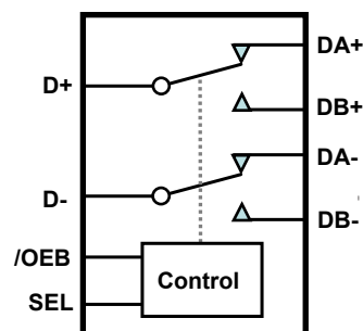
Block Diagram
