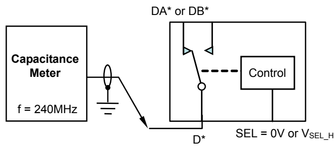
Figure 9. ON Capacitance
