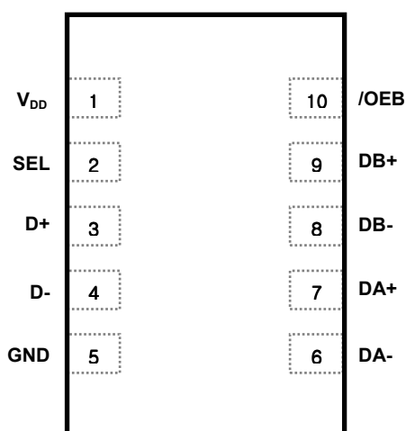
10 pins MSOP (Top View)
