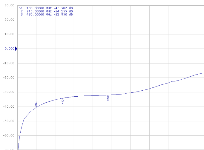
Off Isolation
