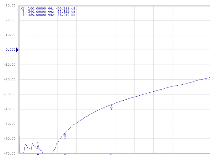
Crosstalk
