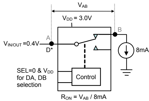
Figure 2. R_{ON} test circuit
