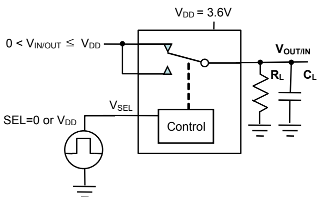
Figure 5. Break-Before-Make time
