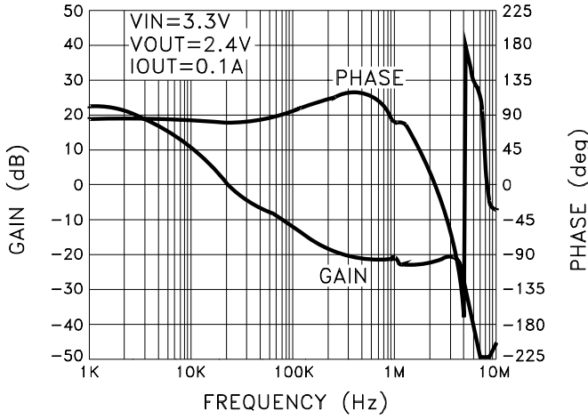
MSK5900RH GAIN AND PHASE vs. FREQUENCY
