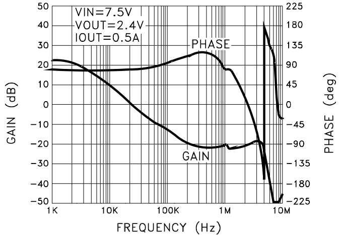
MSK5900RH GAIN AND PHASE vs. FREQUENCY
