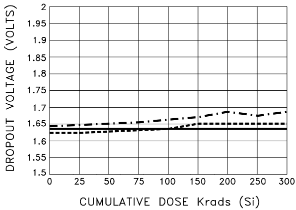
NEGATIVE DROPOUT VOLTAGE
