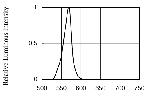
FIG.1 RELATIVE INTENSITY LUMINOUS VS. WAVELENGTH
