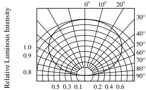
FIG.6 RADIATION DIAGRAM
