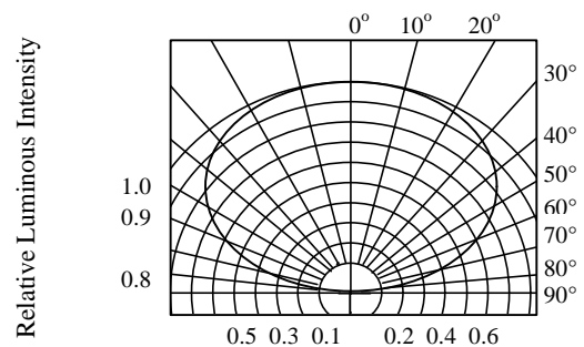
FIG.6 RADIATION DIAGRAM
