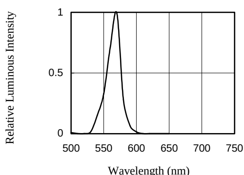
FIG.1 RELATIVE INTENSITY LUMINOUS VS. WAVELENGTH
