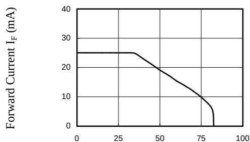
FIG. 3 FORWARD CURRENT VS. AMBIENT TEMPERATURE.
