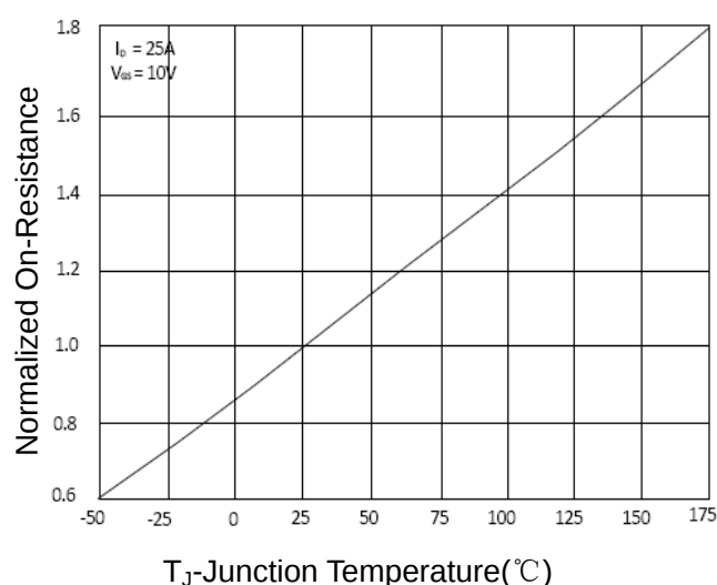
Figure 4 Rdson-Junction Temperature
