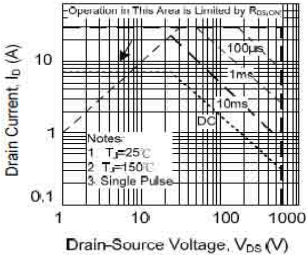
Fig6-1 Maximum Safe Operating Area
