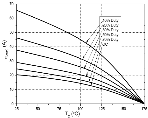
Figure 7. Current Derating
