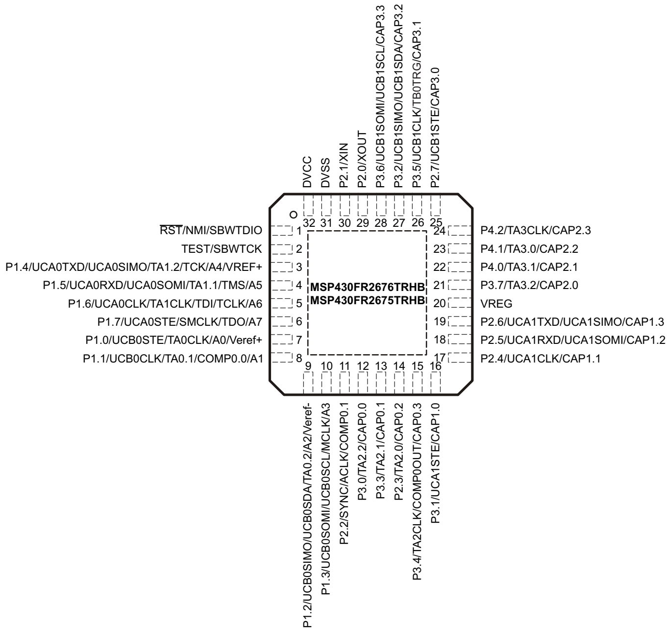
Figure 4-3. 32-Pin RHB Package (Top View)
