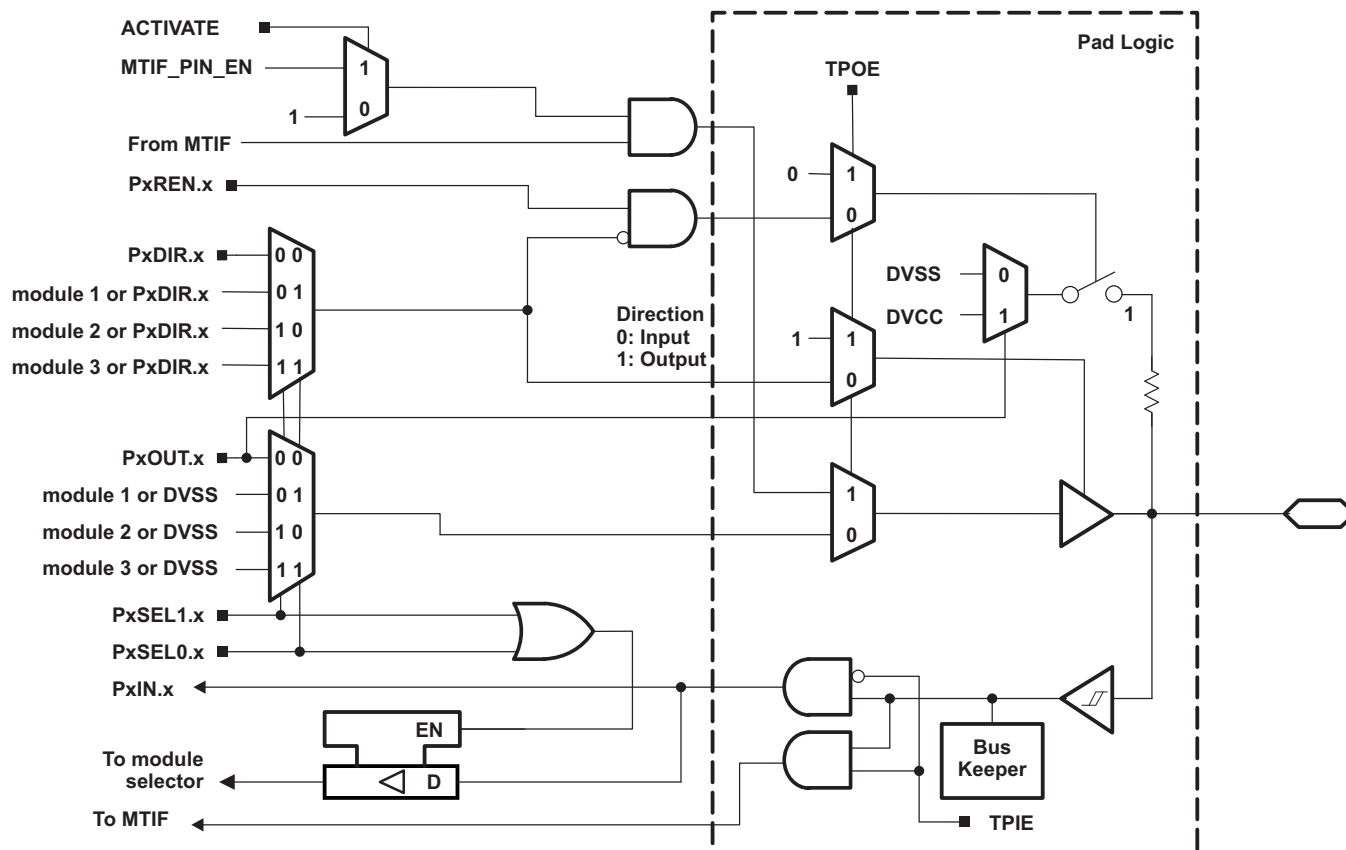
Figure 6-11. Port P3 (P3.1) Diagram
