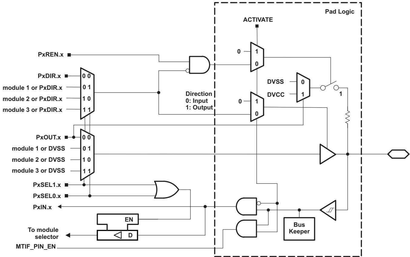
Figure 6-16. Port P4 (P4.0) Diagram
