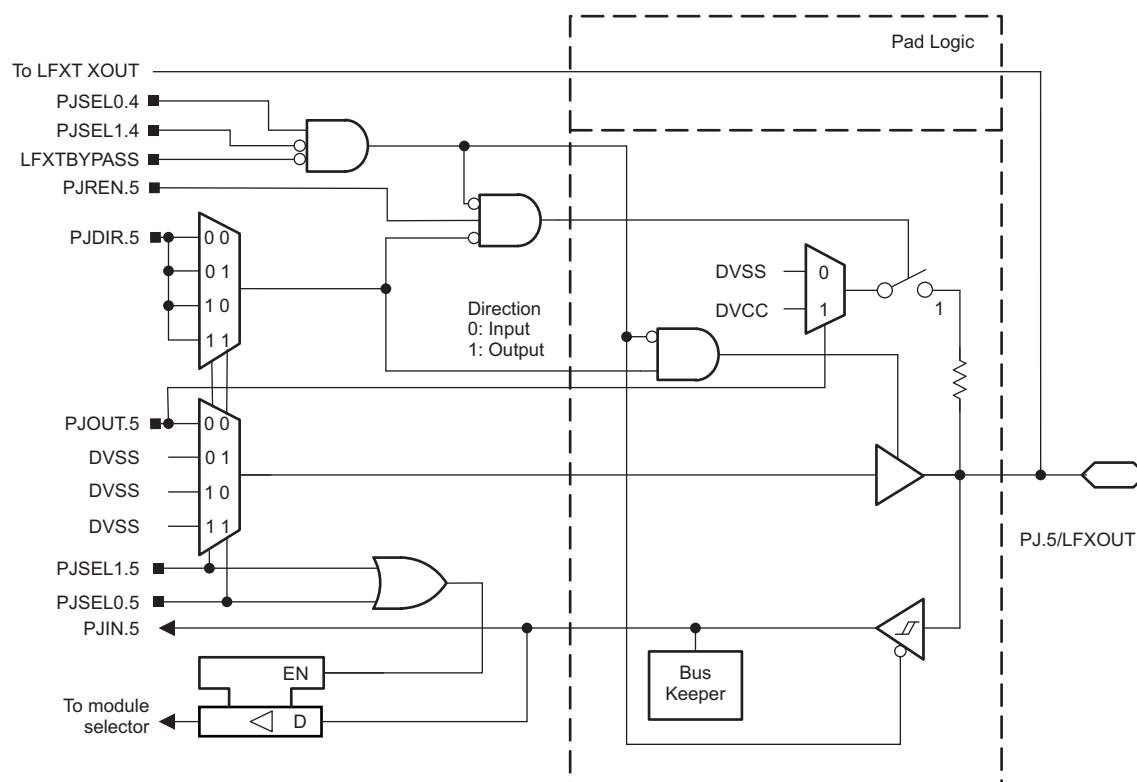
Figure 6-27. Port PJ (PJ.5) Diagram
