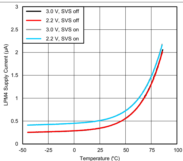
Figure 5-3. LPM4 Supply Current ( I_{LPM4,SVS} ) vs Temperature
