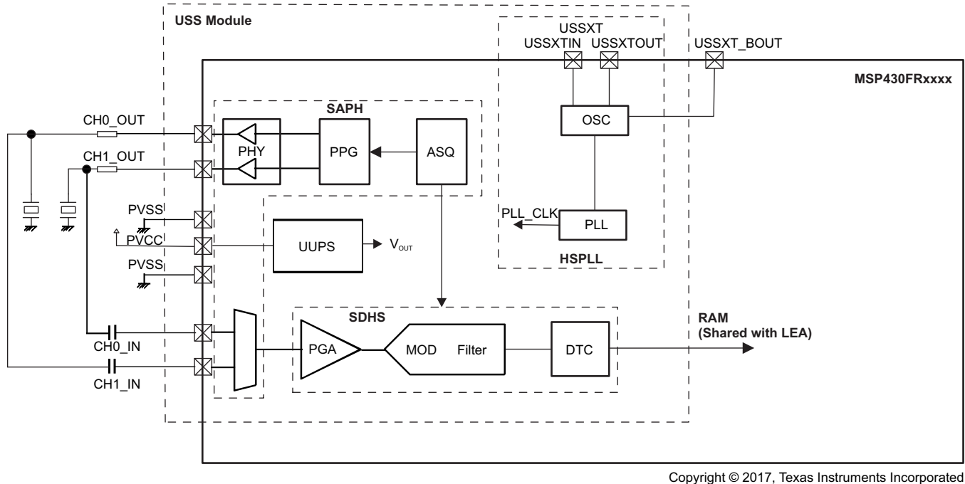
Figure 6-1. USS Subsystem Block Diagram
