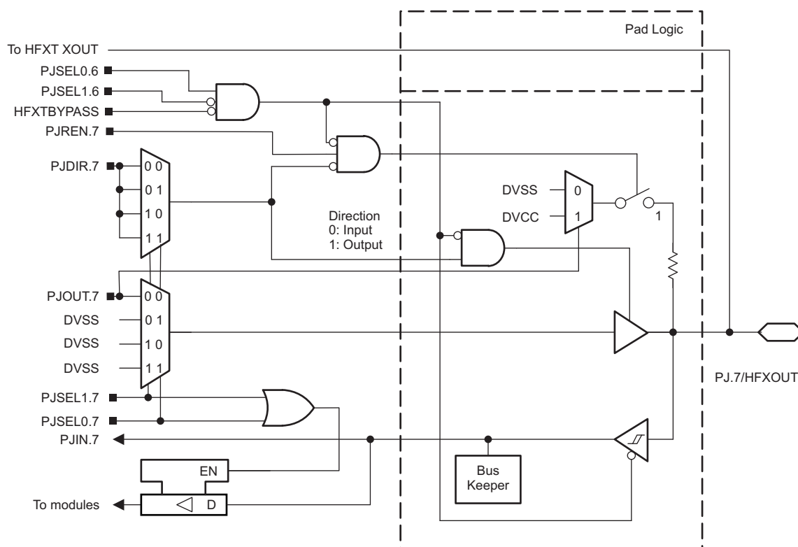
Figure 6-24. Port PJ (PJ.7) Diagram
