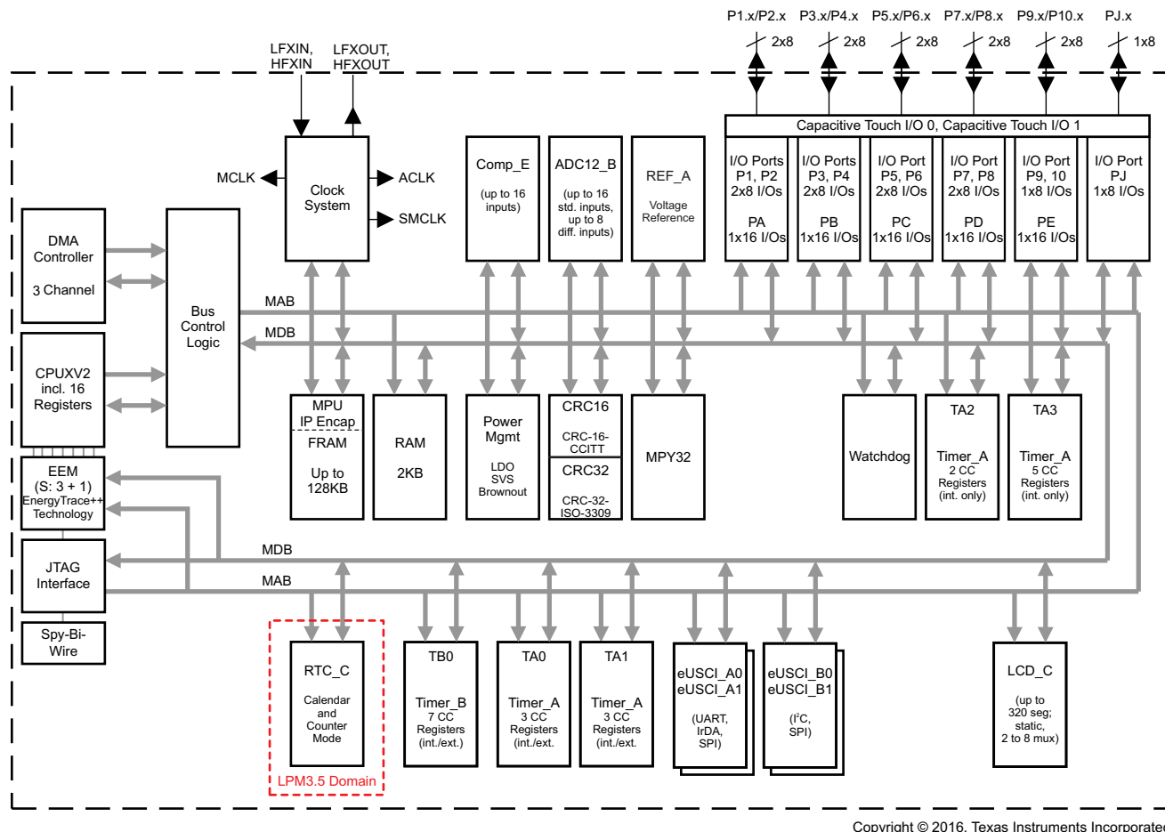
Figure 1-1. Functional Block Diagram – MSP430FR687x, MSP430FR687x1
