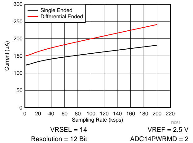
Figure 5-31. Current vs Sampling Rate
