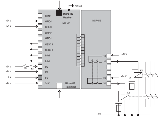
Micro 400 Light Curtain, Automatic Reset, Start/Restart Monitored Output and MSR45E Expansion Module
