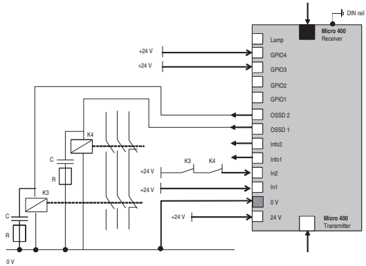
Micro 400 Light Curtain, Automatic Reset, Start/Restart Monitored Output
