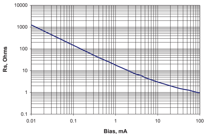
Series Resistance vs. Current (Freq = 500 MHz)
