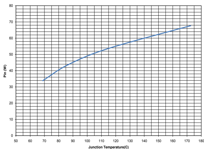
Junction Temperature vs Power with the Backside of Board maintained @ 25^\circ\text{C} Board thickness 62 mils
