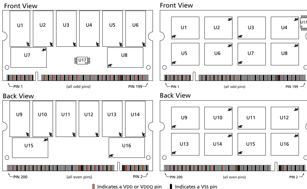
Figure 2: Module Layout
