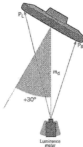
Figure2: Top view of test set-up when the screen is rotated \pm 30 degrees. The +rotation is defined clockwise.
