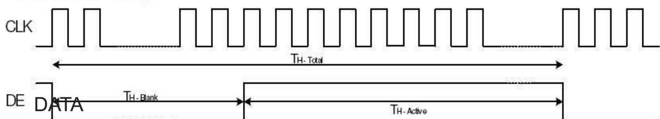
Horizontal Input Timing
