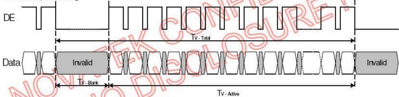
Vertical Input Timing
