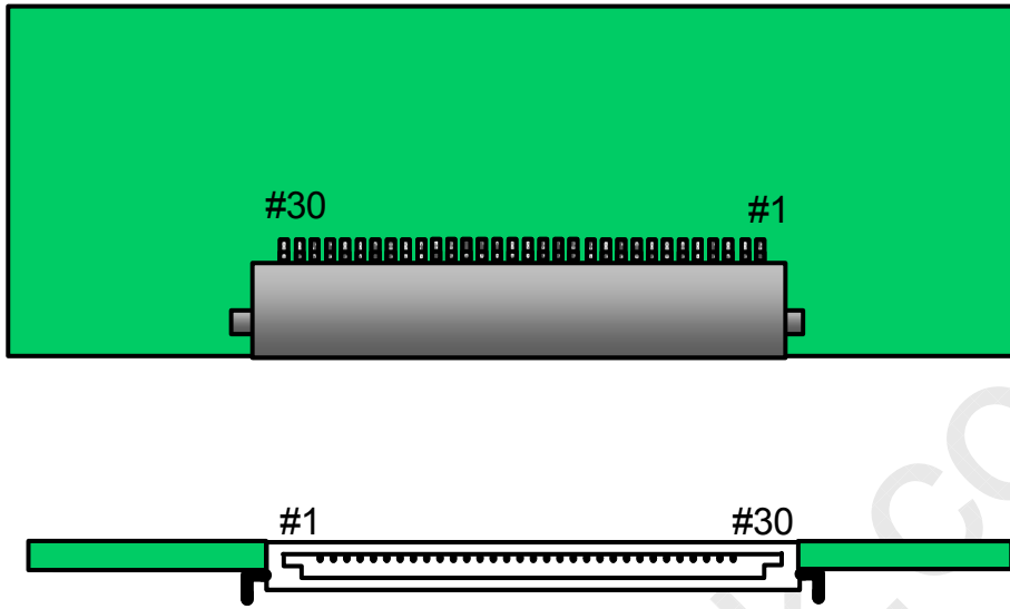
Rear view of LCM
