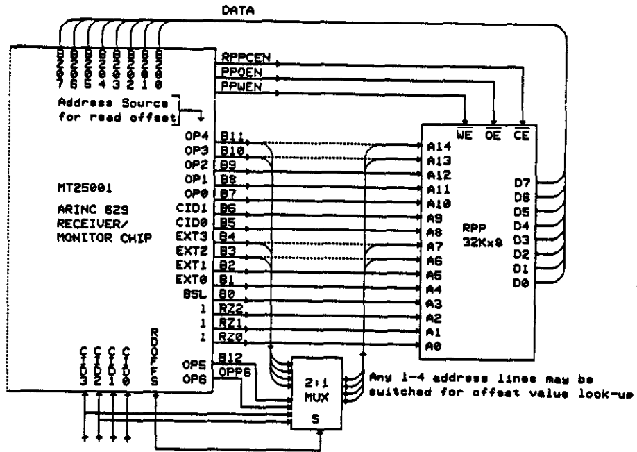
Fig 2. RPP CONNECTIONS FOR SPECIAL OFFSET VALUE ADDRESSING
