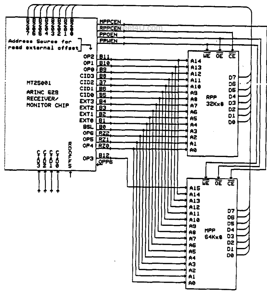
Fig 3. FULL RPP/MPP CONNECTION SCHEME
