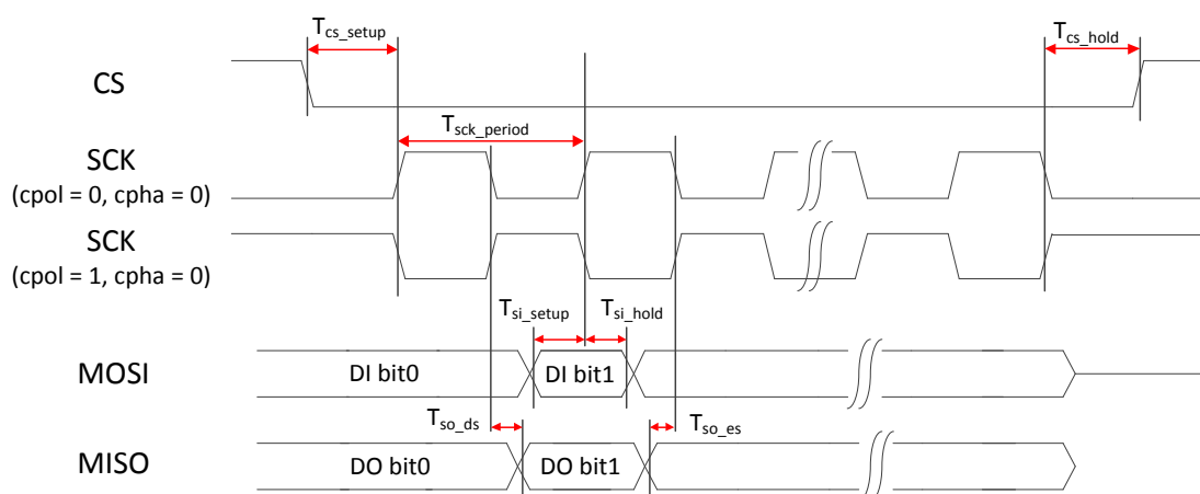
Figure 8-3. SPI slave interface timing diagram (CPHA=0)
