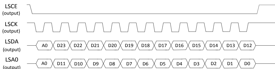
Figure 8-23. 2-data-pin mode write (A0+12-bit)
