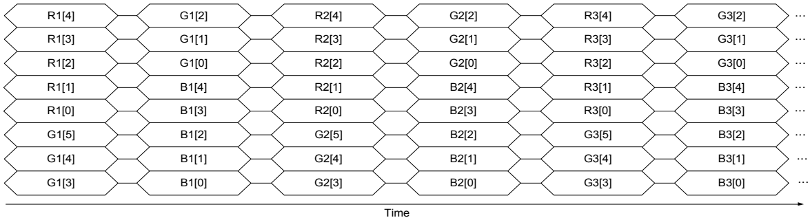
Figure 8-30. Pixel format of RGB565
