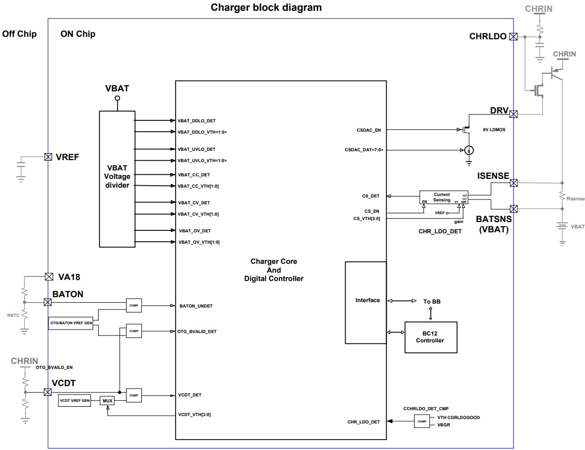
Figure 4-4. PCHR schematics
