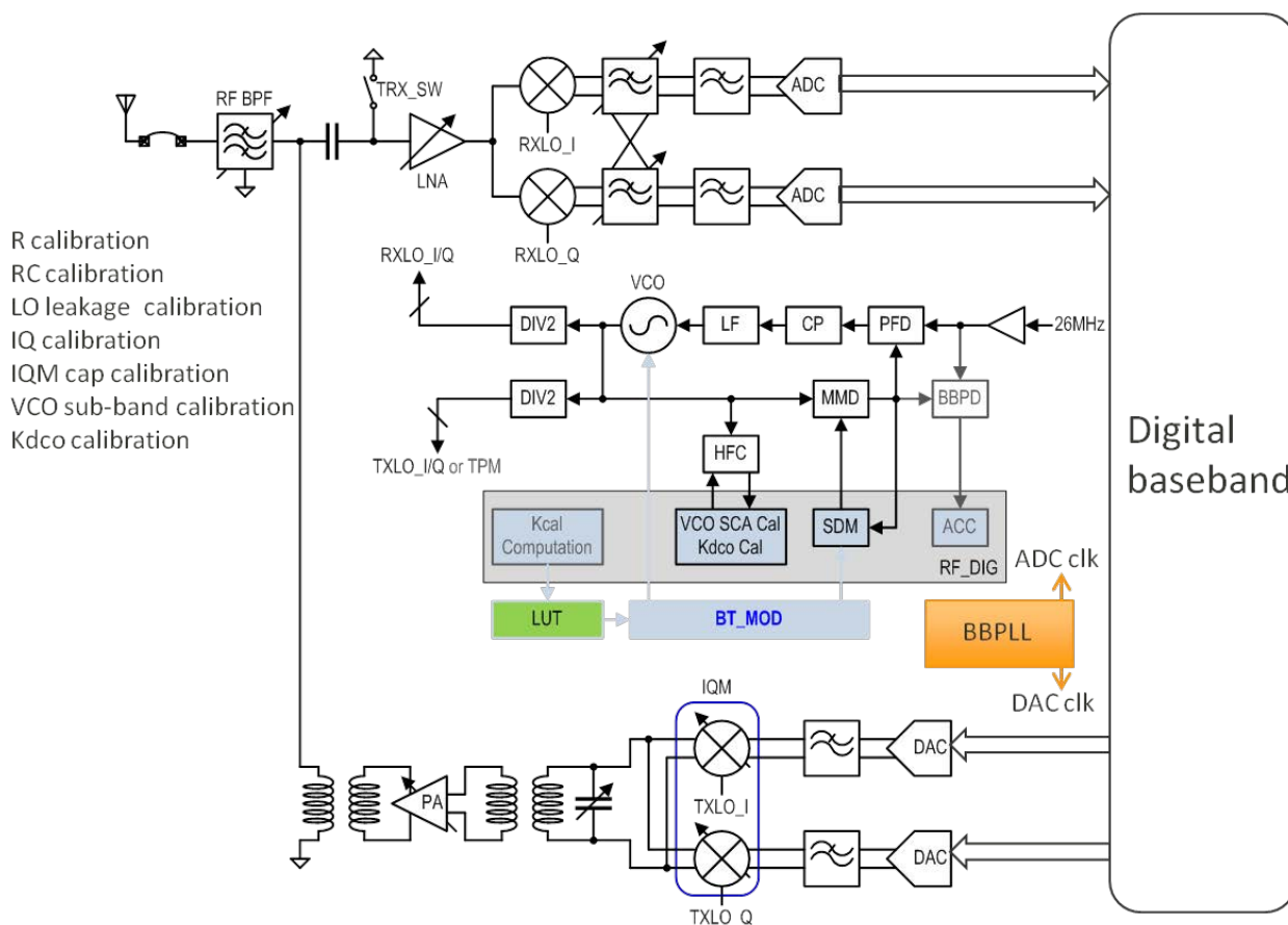
Figure 3-1. Bluetooth RF transceiver system
