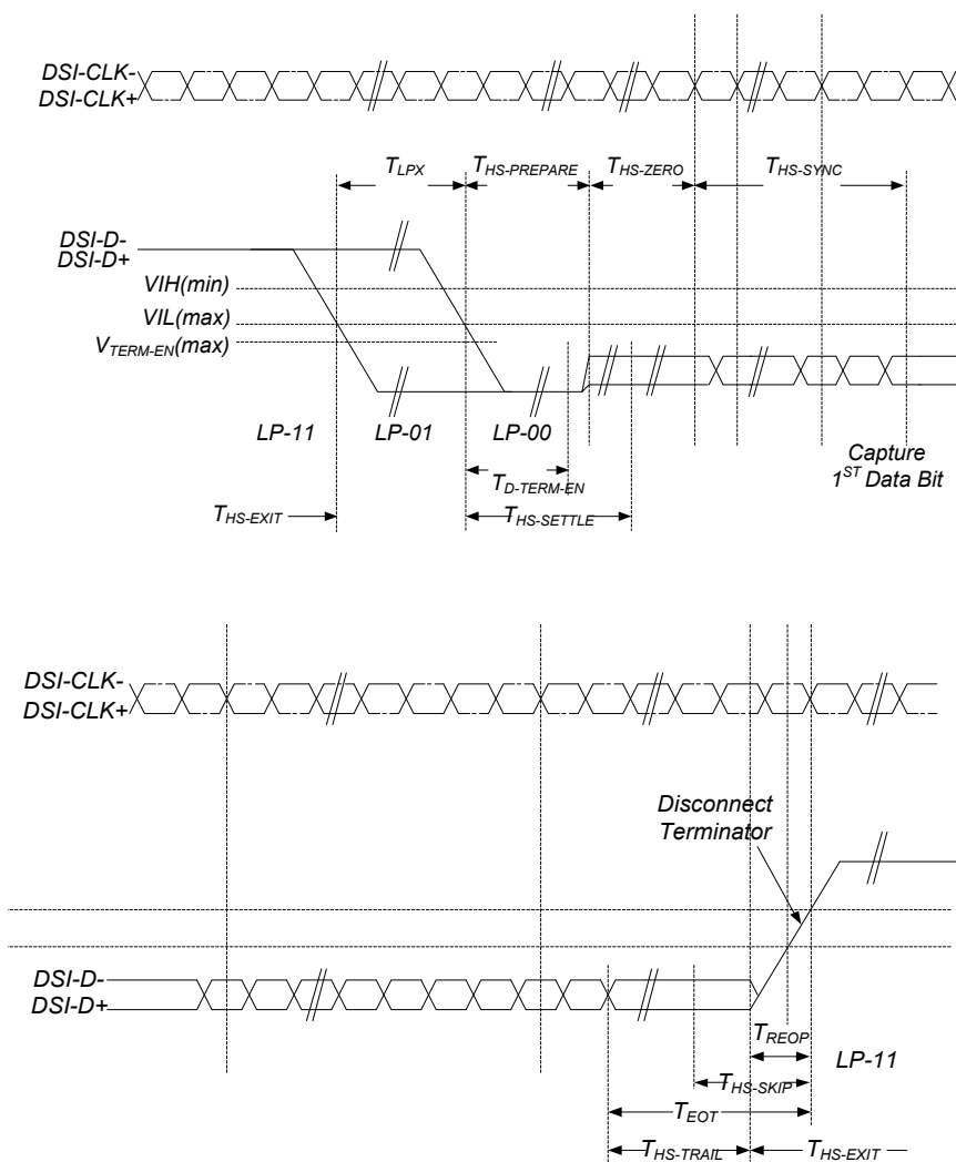
Figure 8-25. HS data transmission in bursts
