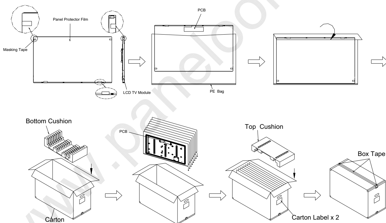
Fig. 8.1 Packing method
