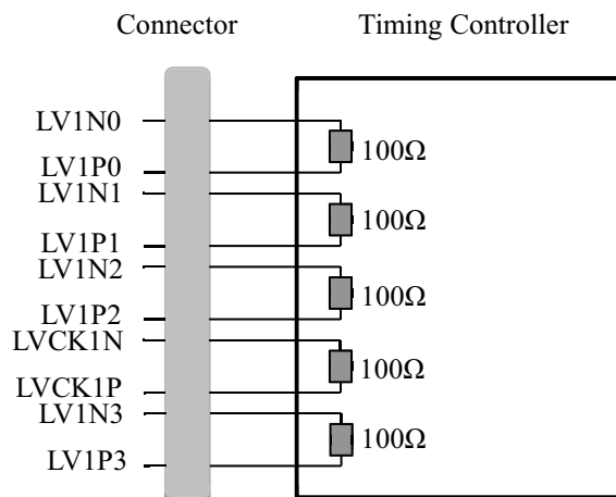
Fig. 5.3 Block diagram of interface
