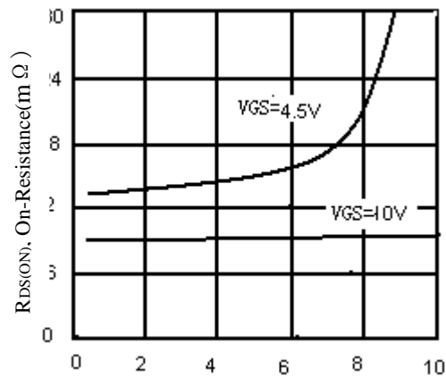
I_D -DrainCurrent (A)
