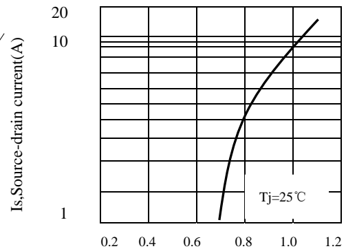
VSD, Body Diode Forward Voltage Figure8. Body Diode Forward Voltage
