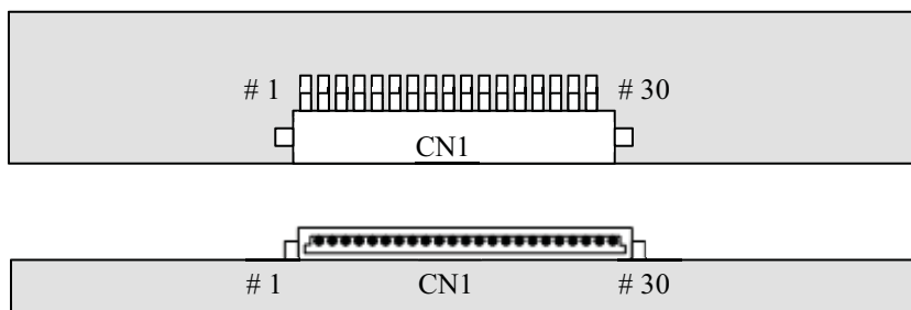
Fig. 4.1 LVDS connector direction sketch map
