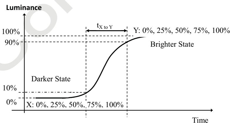
Fig. 6.4 The definition of t_{X \text{ to } Y}
