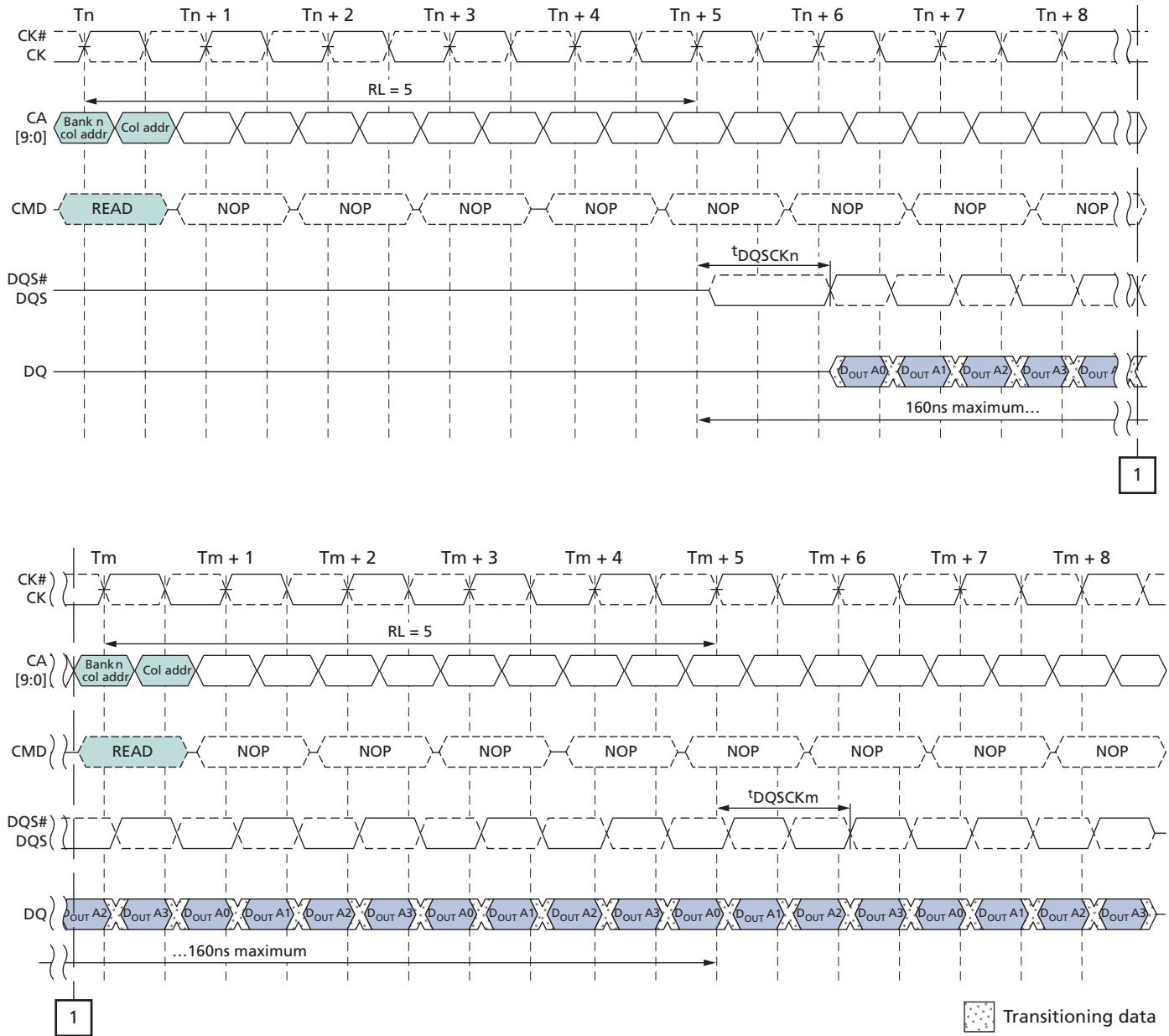
Figure 35: t_{DQSKDS} Timing
