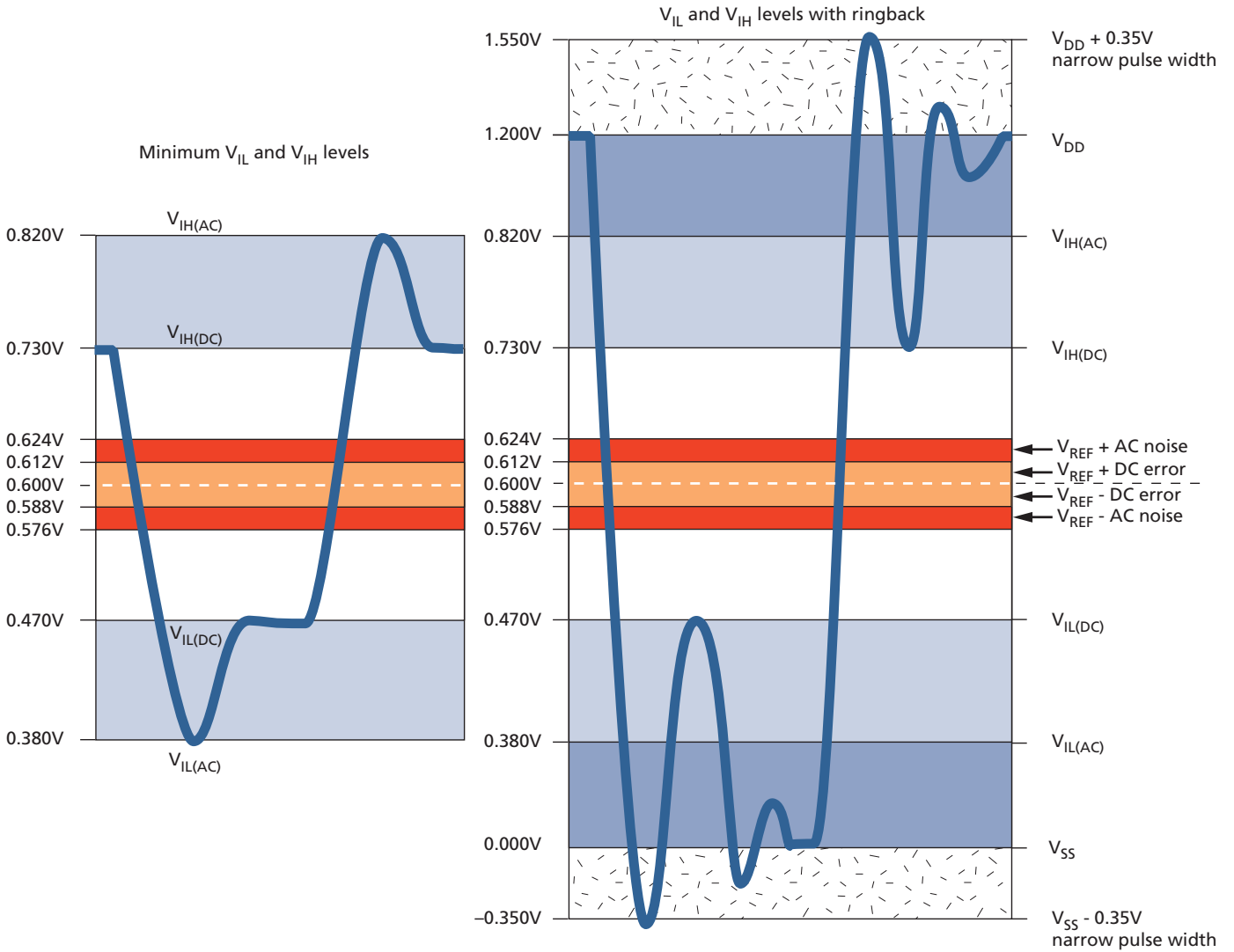
Figure 83: LPDDR2-466 to LPDDR2-1066 Input Signal
