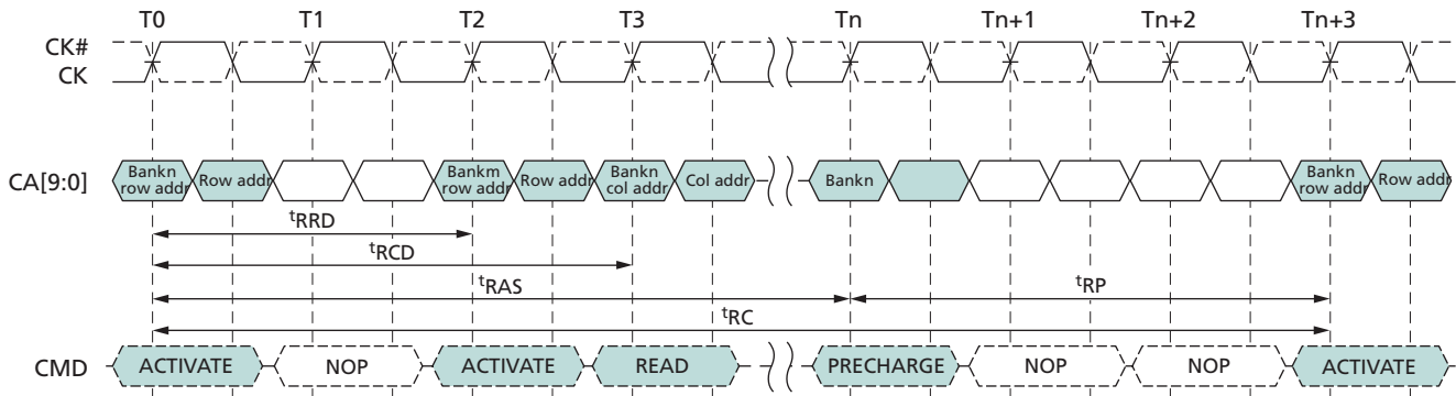
Figure 27: ACTIVATE Command
