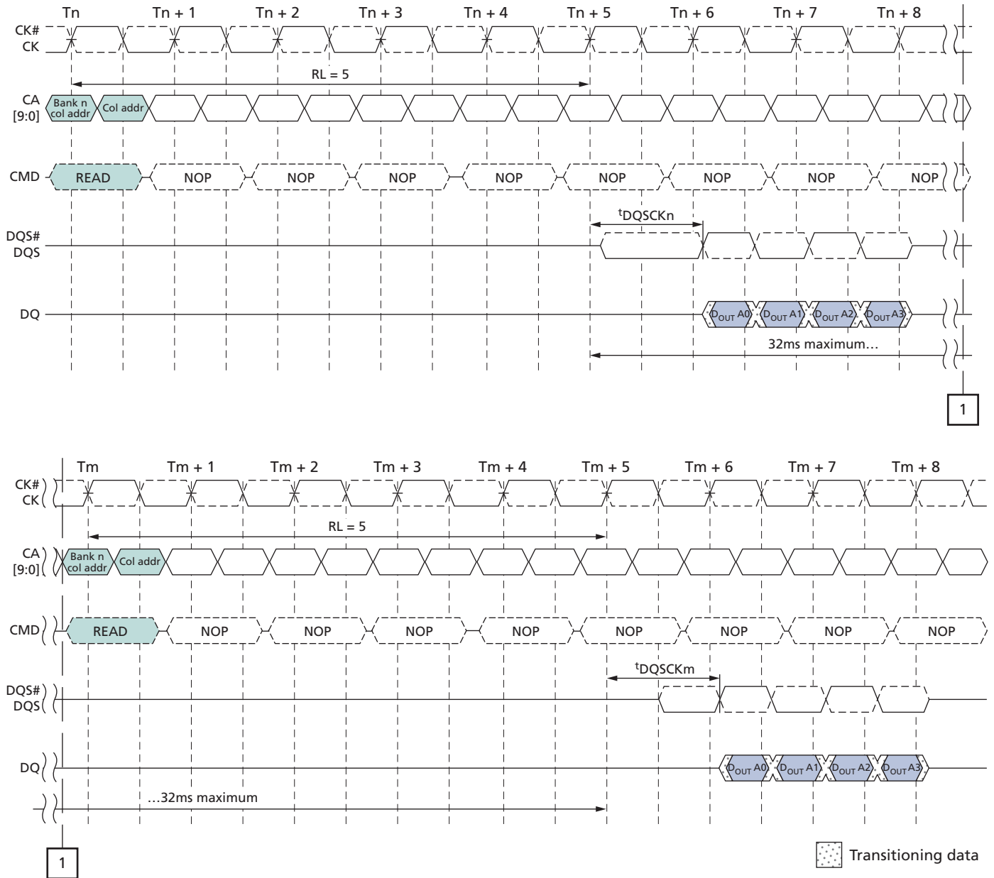
Figure 33: t_{DQSKDL} Timing
