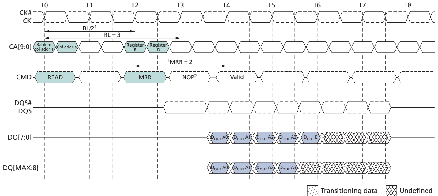
Figure 62: READ to MRR Timing – RL = 3, t^{\text{MRR}} = 2
