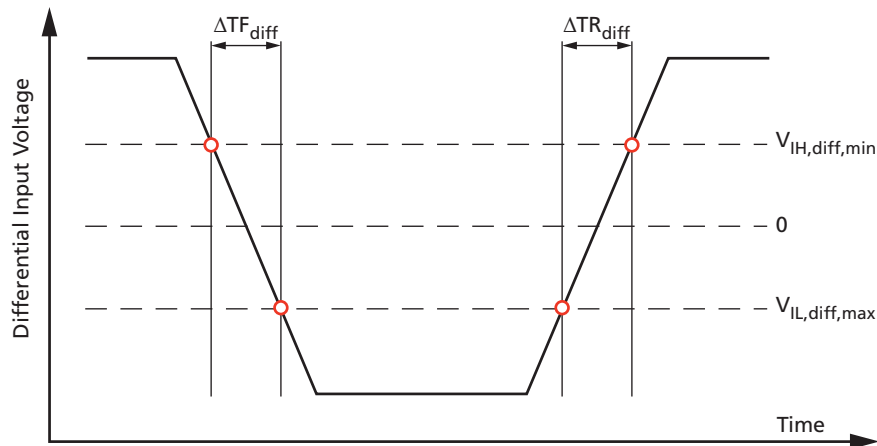
Figure 88: Differential Input Slew Rate Definition for CK, CK#, DQS, and DQS#
