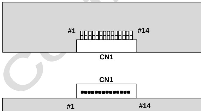
Fig. 5.2 Power input connector direction sketch map
