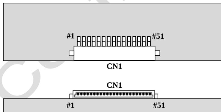
Fig. 5.1 LVDS connector direction sketch map
