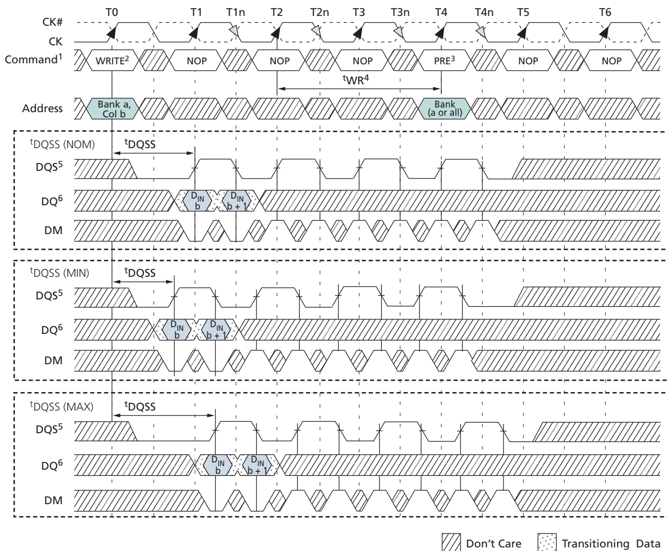
Figure 42: WRITE-to-PRECHARGE – Interrupting
