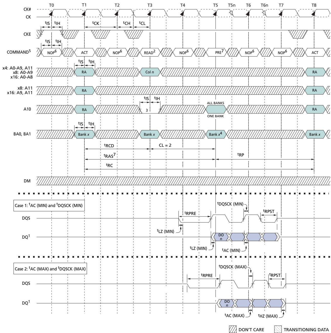
Figure 47: Bank Read – Without Auto Precharge
