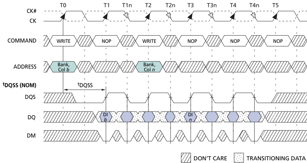
Figure 20: Consecutive WRITE to WRITE
