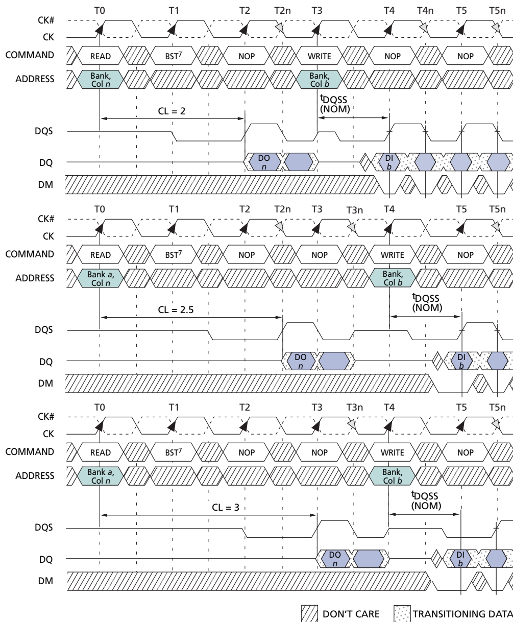
Figure 16: READ to WRITE
