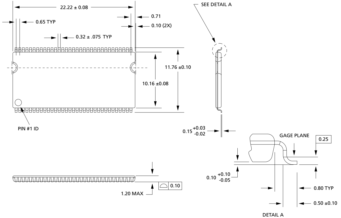
Figure 52: 66-Pin Plastic TSOP (400 mil)
