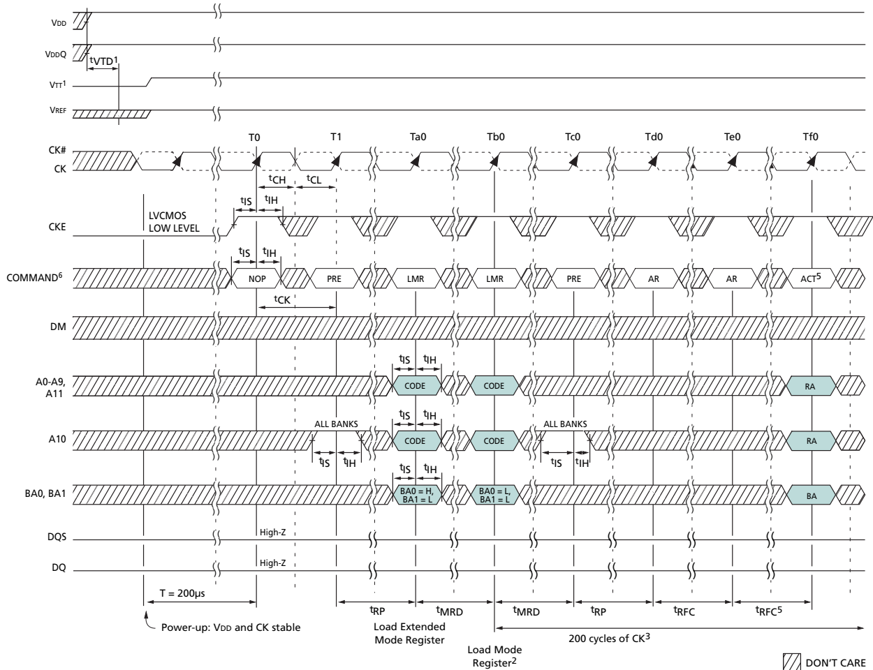
Figure 43: Initialize and Load Mode Registers
