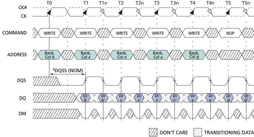
Figure 22: Random WRITE Cycles
