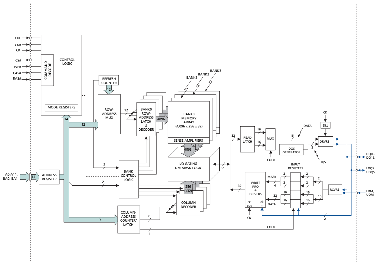
Figure 3: 8 Meg x 16
