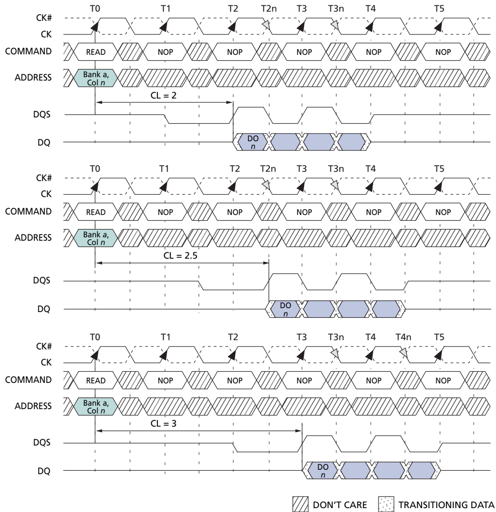
Figure 11: READ Burst
