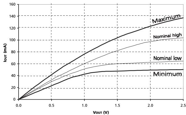
Figure 35: Full Drive Pull-Up Characteristics
