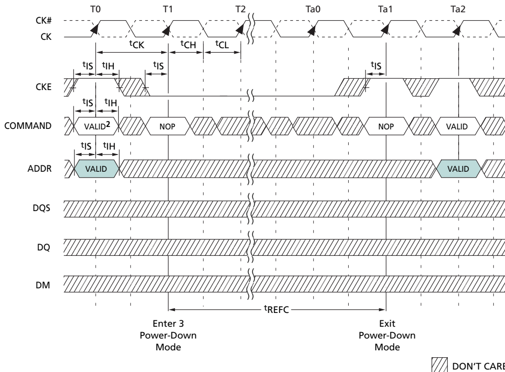
Figure 44: Power-Down Mode
