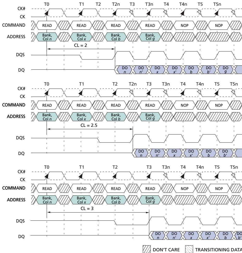
Figure 14: Random READ Accesses
