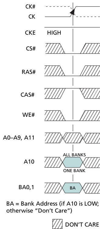
Figure 29: PRECHARGE Command
