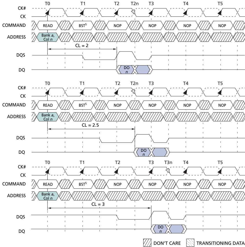
Figure 15: Terminating a READ Burst
