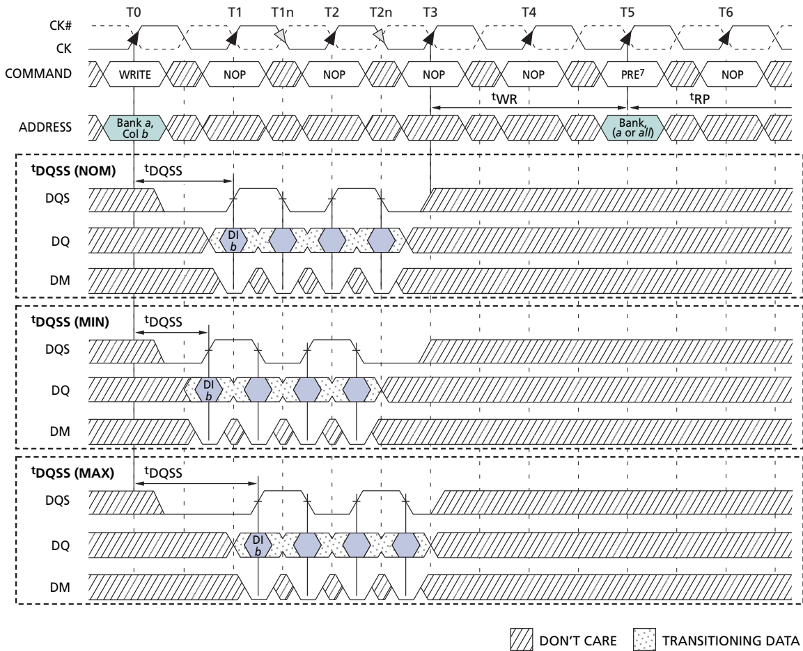
Figure 26: WRITE to PRECHARGE - Uninterrupting
