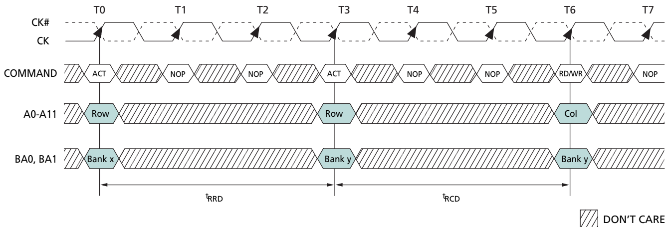
Figure 9: Example: Meeting t_{RCD} (t_{RRD}) \text{ MIN} When 2 < t_{RCD} (t_{RRD}) \text{ MIN} / t_{CK} \leq 3
