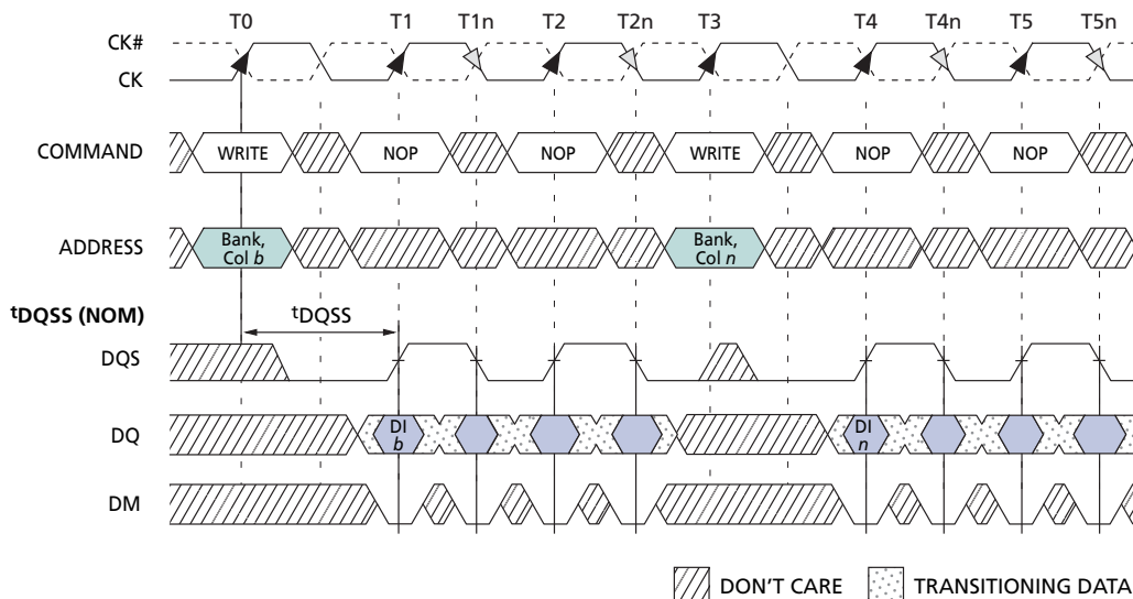
Figure 21: Nonconsecutive WRITE to WRITE
