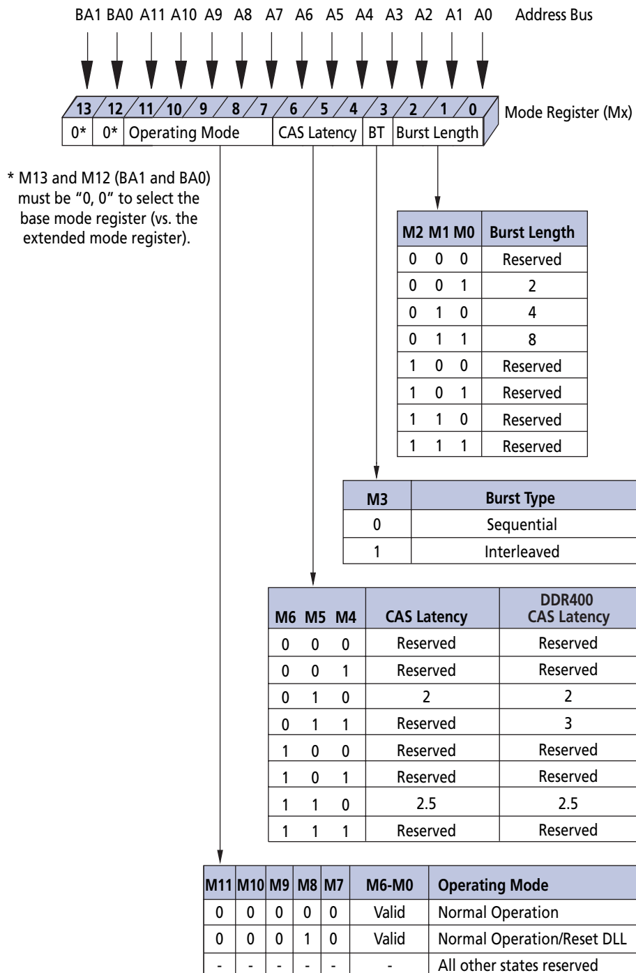
Figure 5: Mode Register Definition
