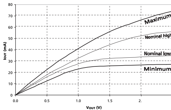
Figure 37: Reduced Drive Pull-Up Characteristics
