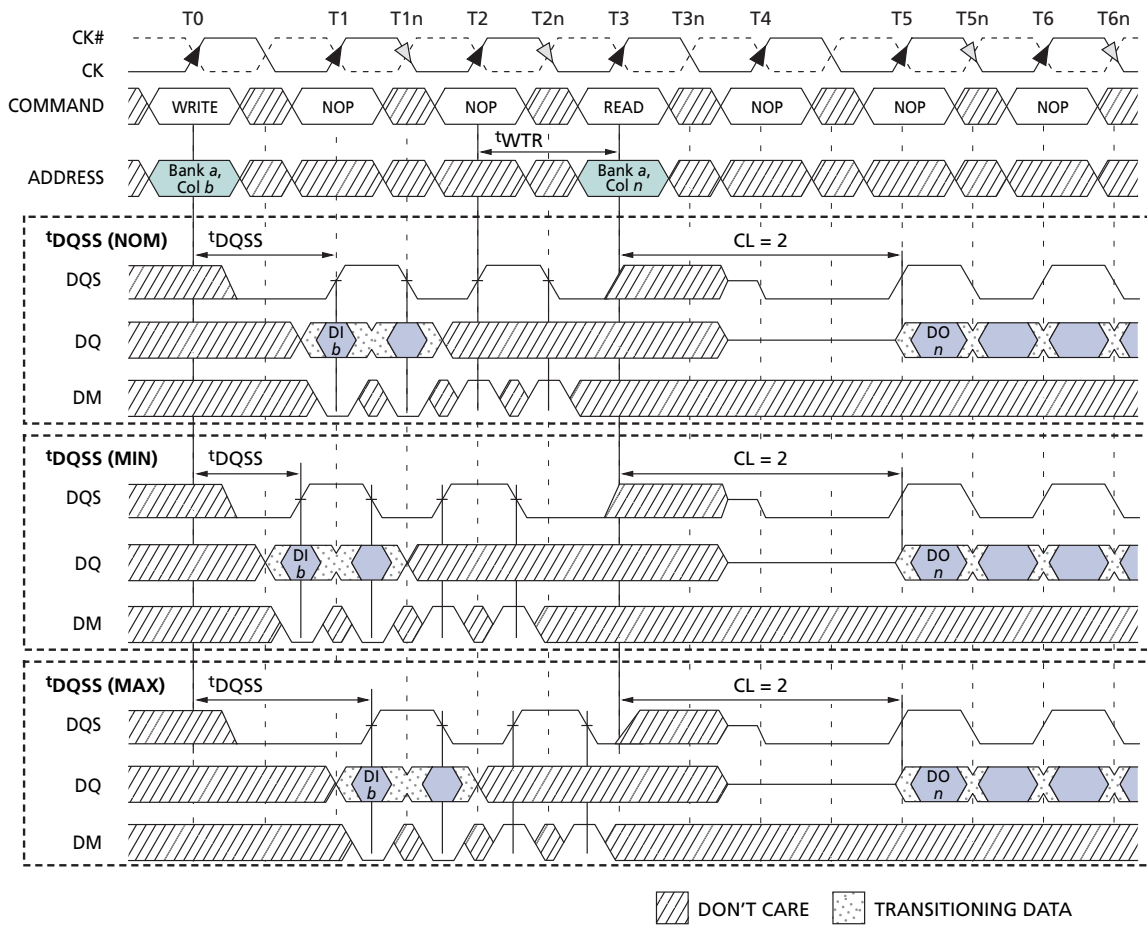
Figure 24: WRITE to READ - Interrupting
