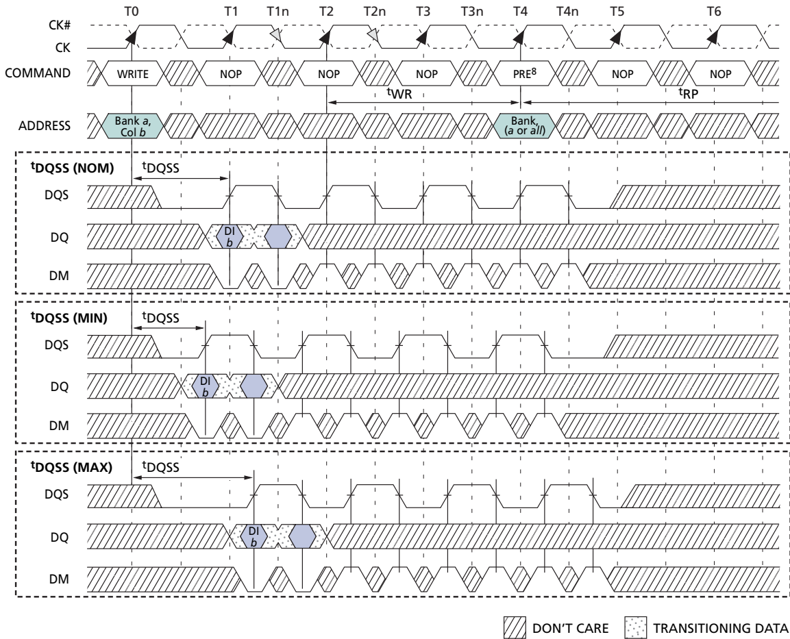
Figure 27: WRITE to Precharge – Interrupting
