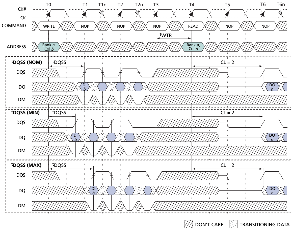
Figure 23: WRITE to READ - Uninterrupting
