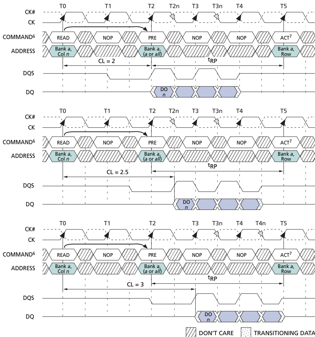
Figure 17: READ to PRECHARGE
