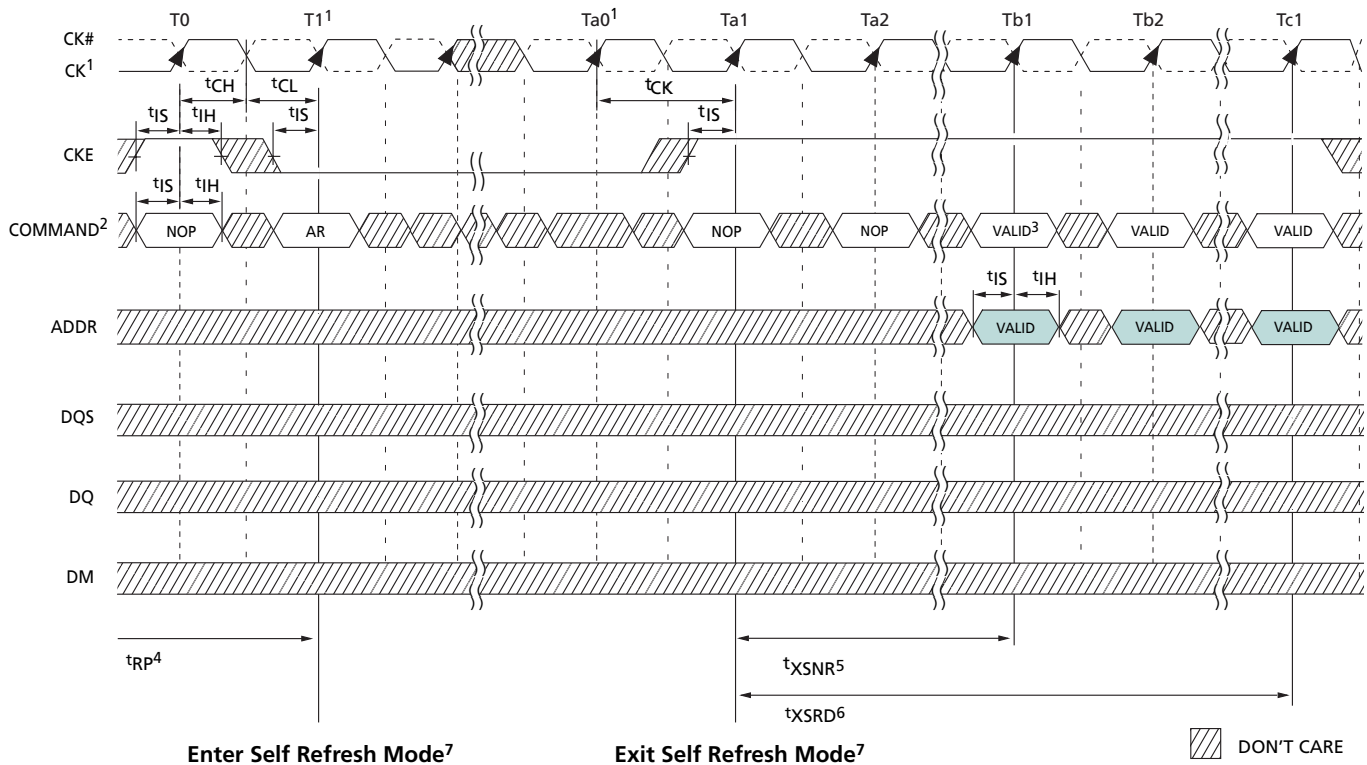
Figure 46: Self Refresh Mode
