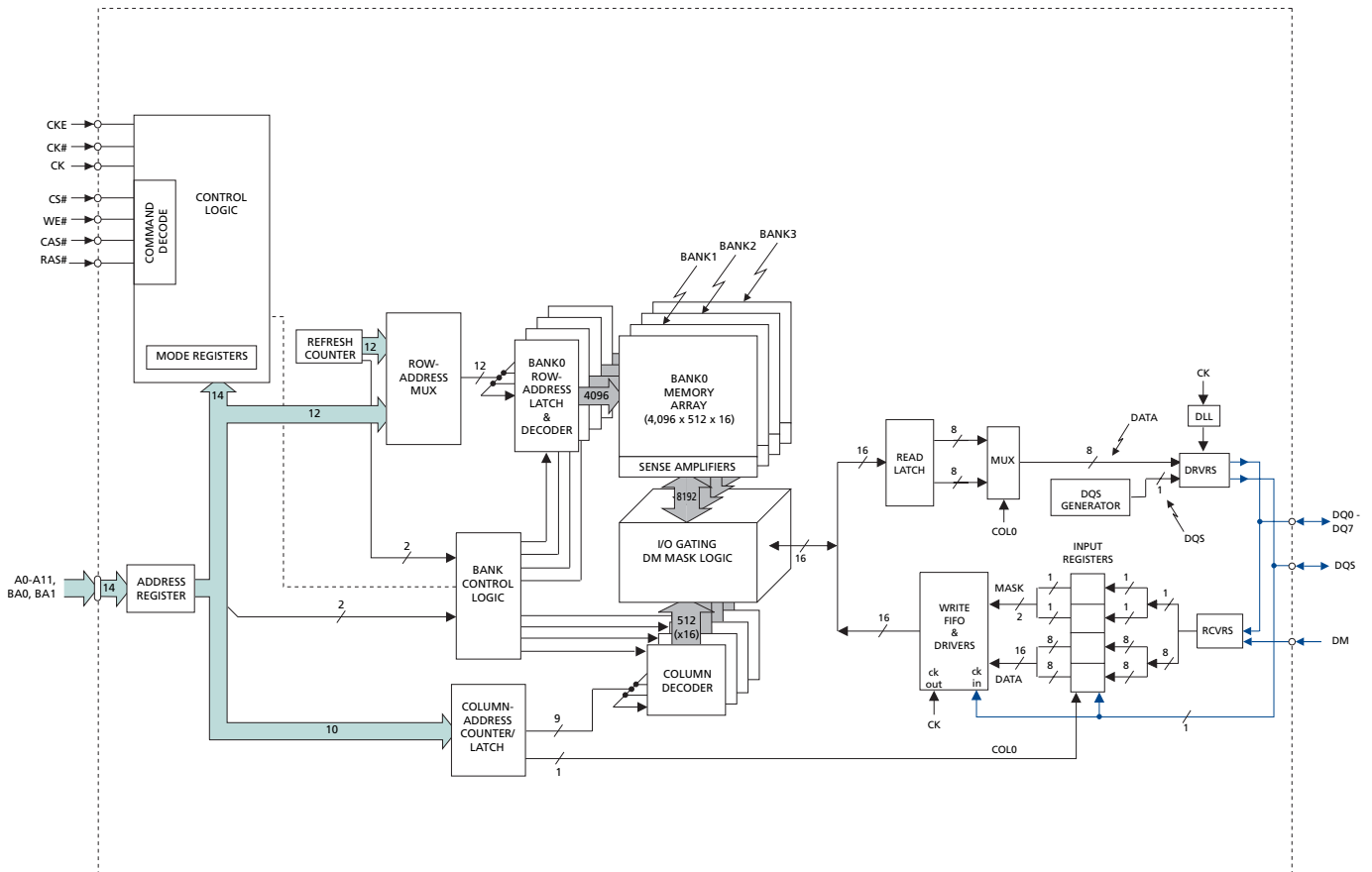
Figure 2: 16 Meg x 8
