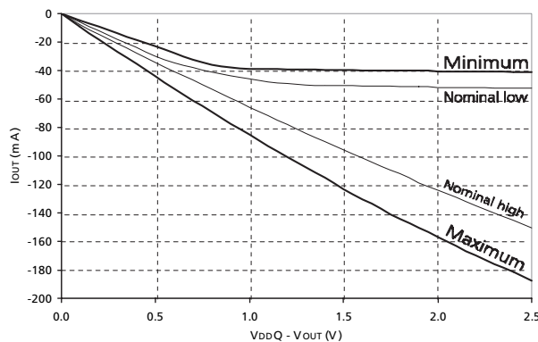
Figure 35: Full Drive Pull-Up Characteristics
