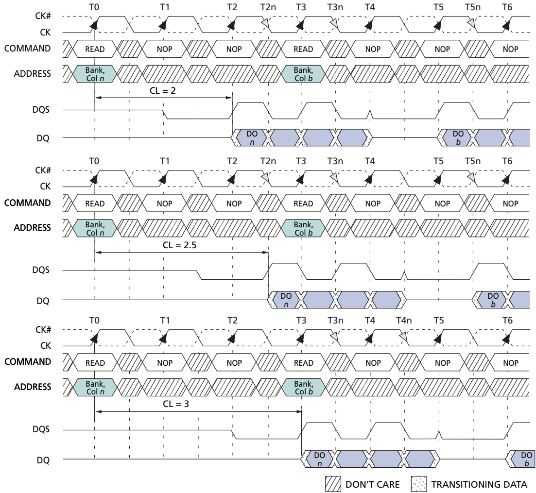
Figure 13: Nonconsecutive READ Bursts
