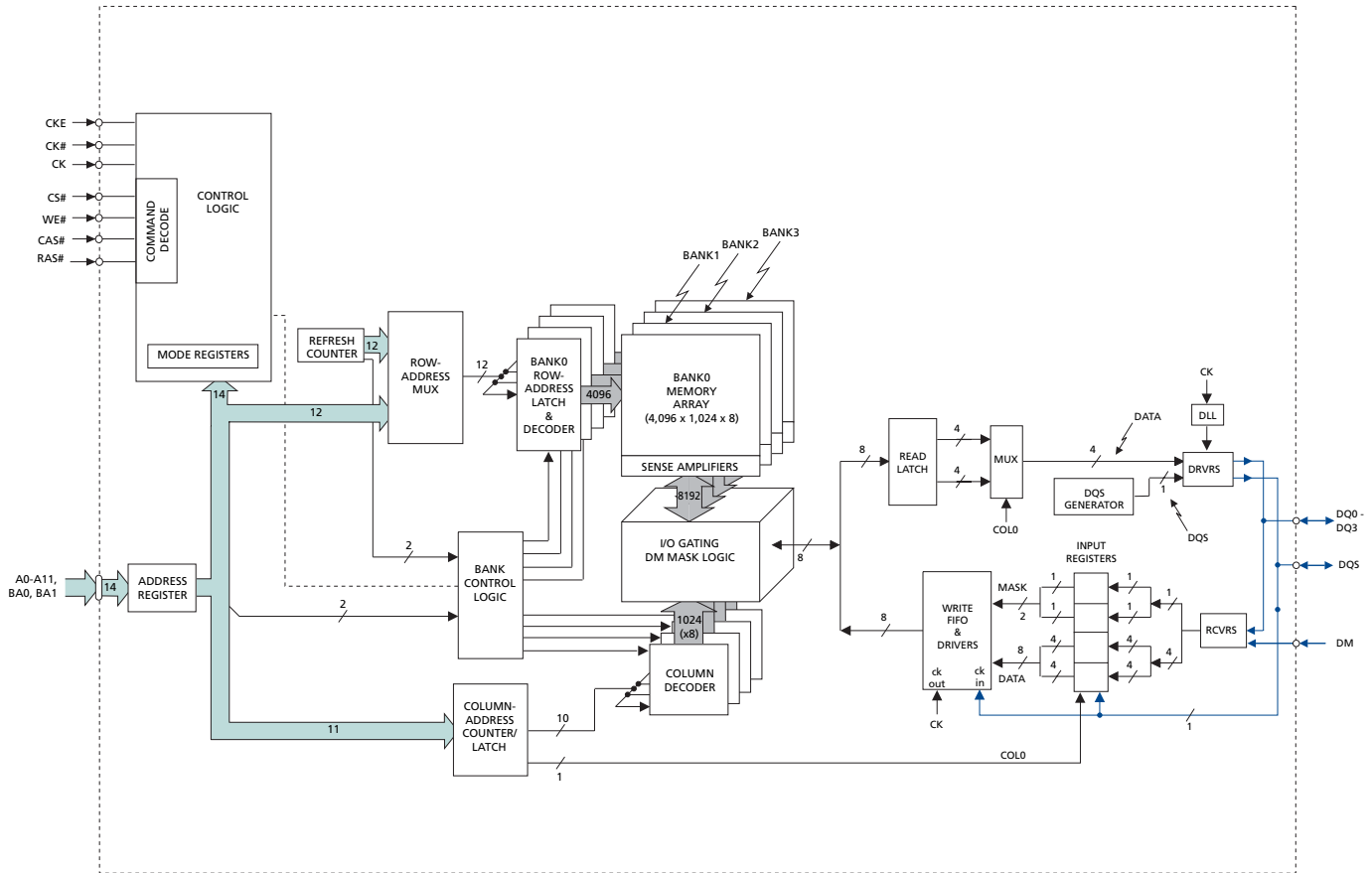
Figure 1: 32 Meg x 4
