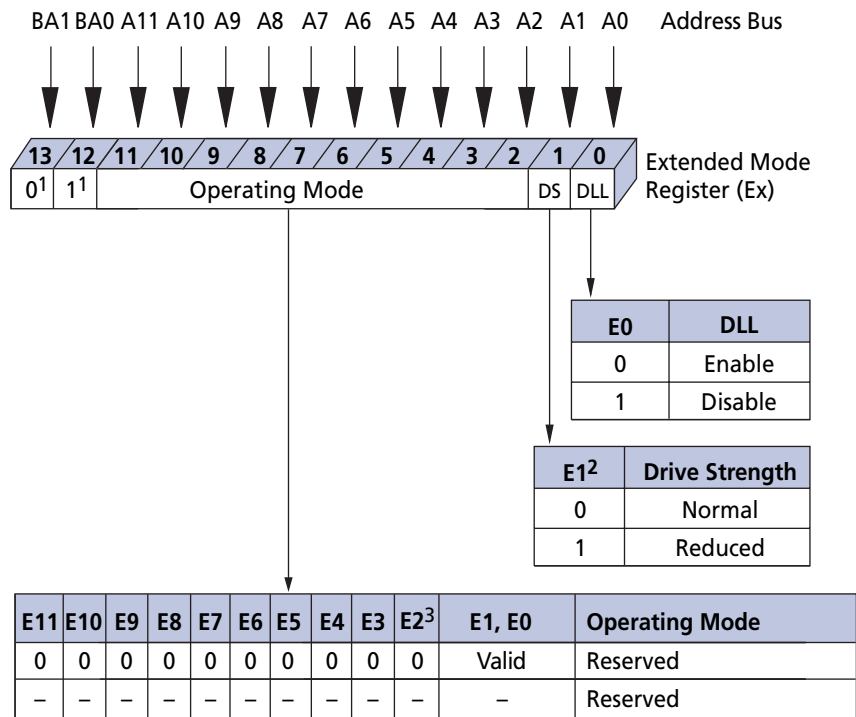
Figure 7: Extended Mode Register Definition
