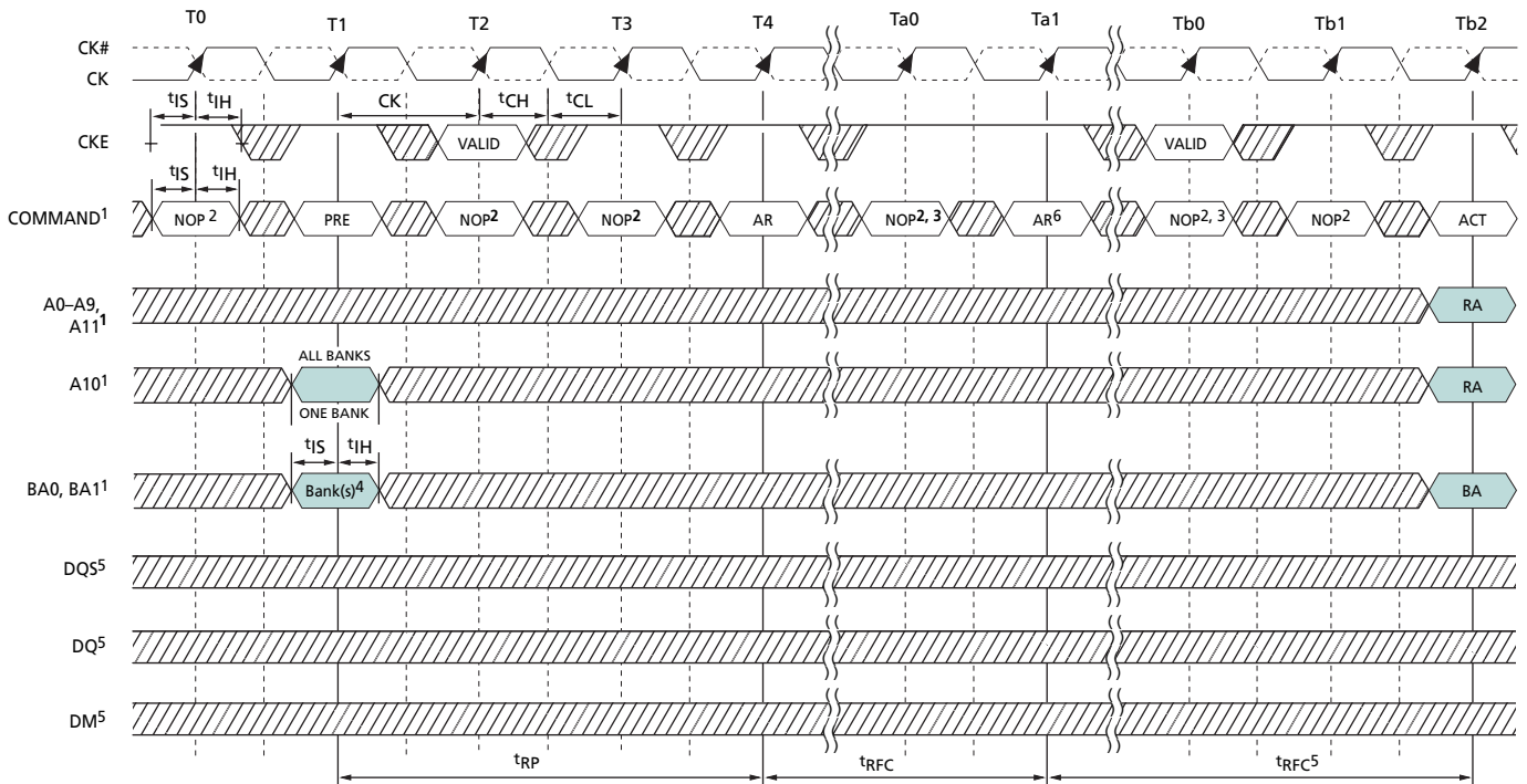
Figure 45: Auto Refresh Mode
