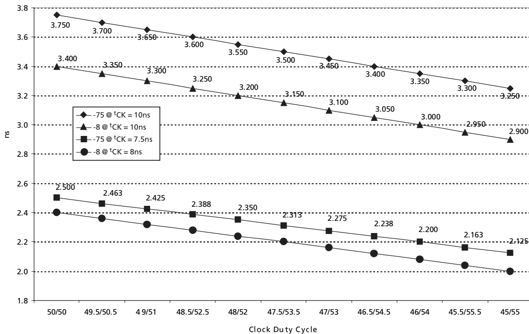
Figure 33: Derating Data Valid Window ( t_{QH} - t_{DQSQ} ) Examples are for speed grades through -75
