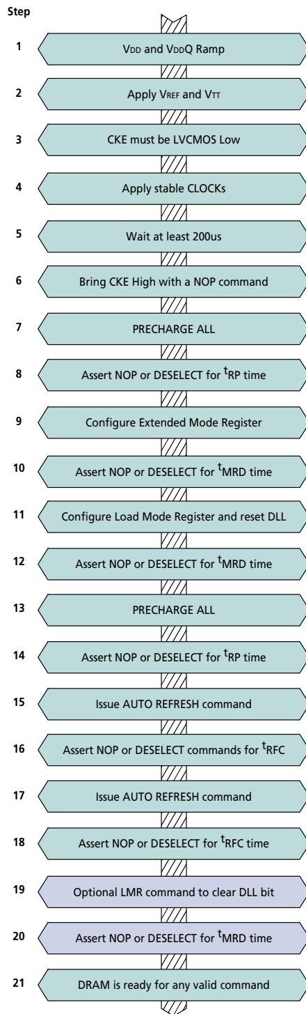
Figure 42: Initialization Flow Diagram
