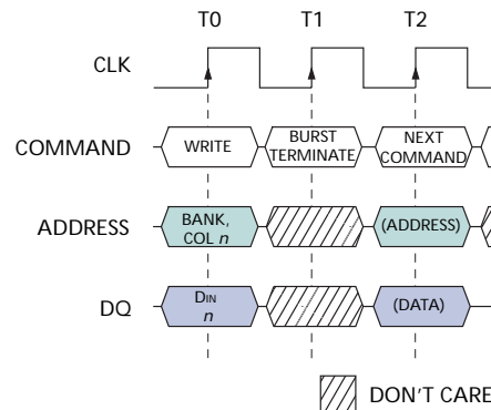
Figure 22: Terminating a WRITE Burst
