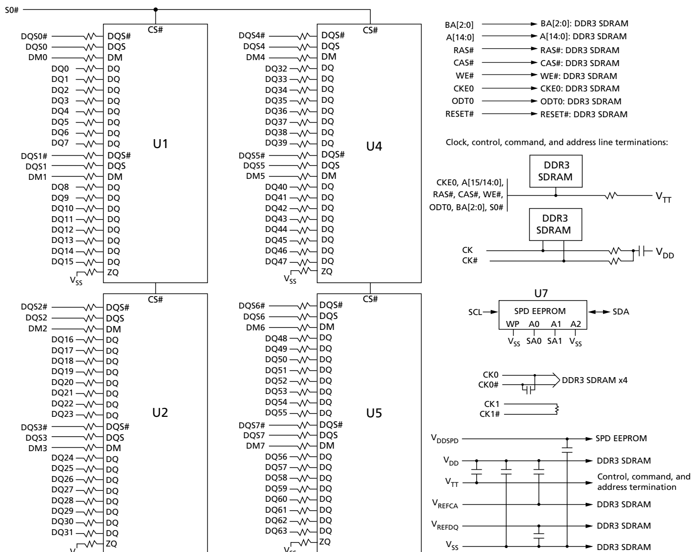
Figure 3: Functional Block Diagram (PCB 2085, R/C-C3)
