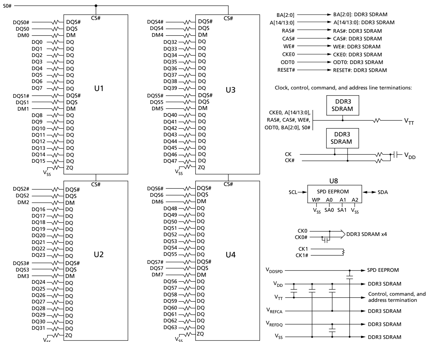
Figure 2: Functional Block Diagram (PCB 0698, R/C-C)
