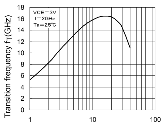
f_T-I_C
