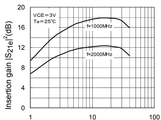
|S_{21e}|^2-I_C
