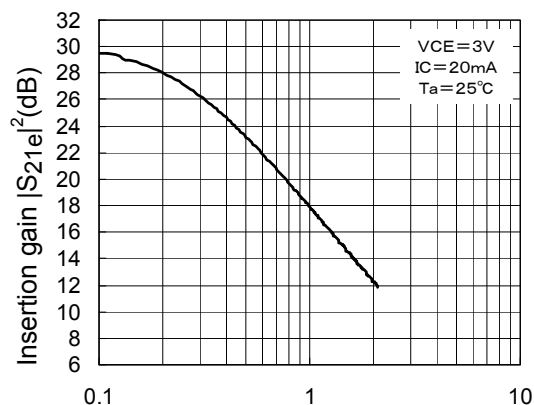
Frequency (GHz)
