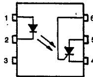
PIN CONFIGURATIONS (TOP VIEW)
