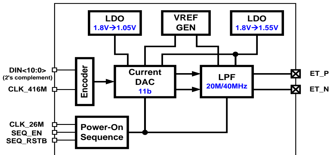
Figure 2-15. Block diagram of ETDAC
