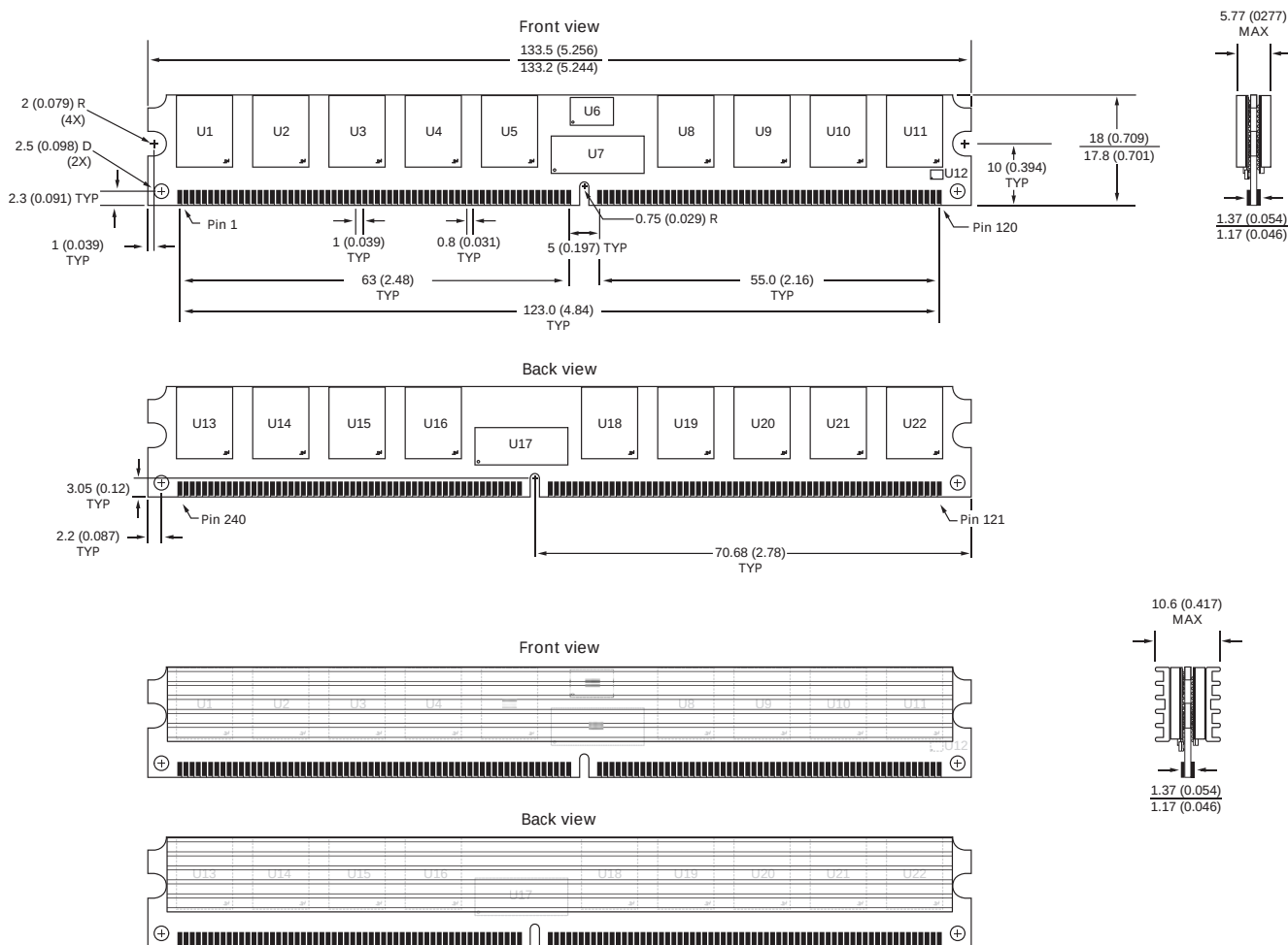
Figure 3: 240-Pin DDR2 VLP RDIMM
