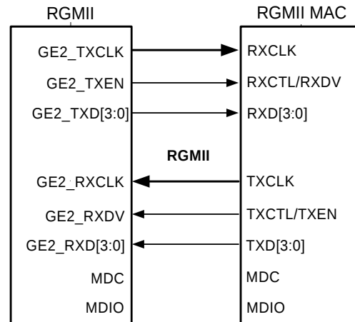
Figure 2-4 RGMII → RGMII MAC
