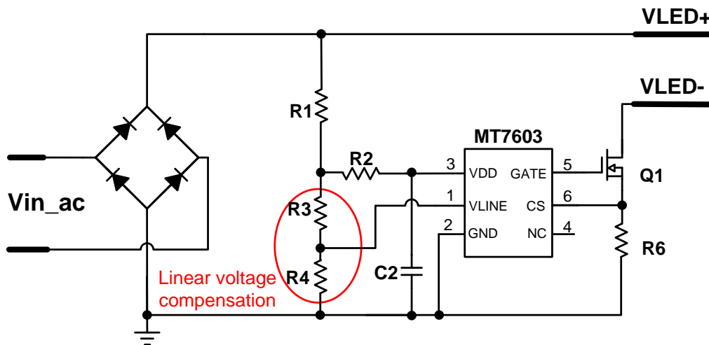
Fig.3 Linear compensation application circuit
