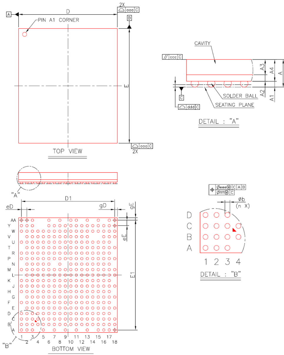
Figure 4-1 Package Dimension
