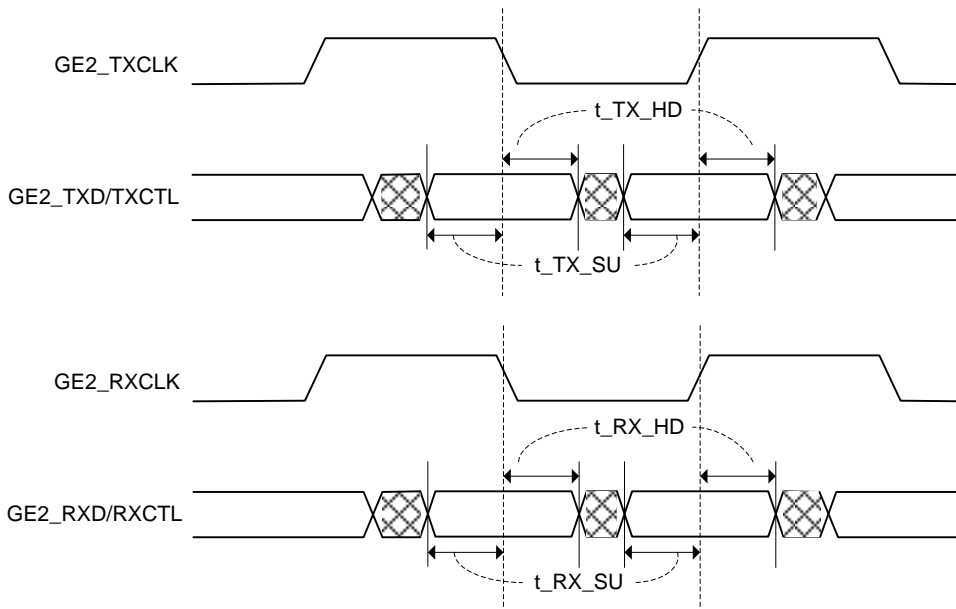
Figure 3-1 RGMII Timing
