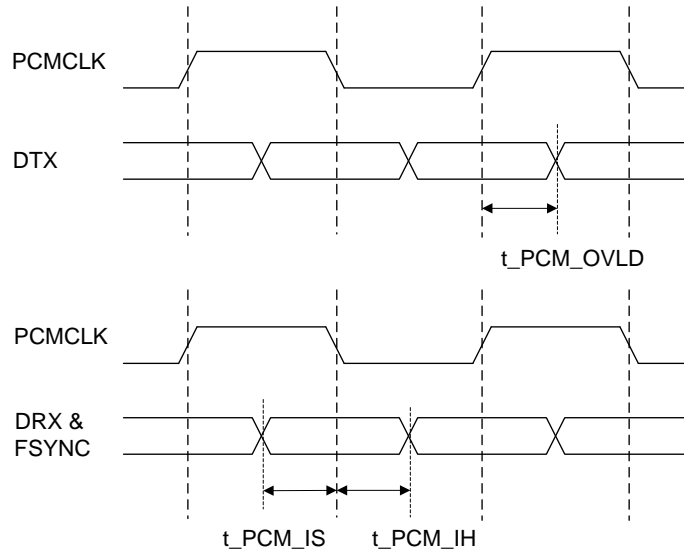
Figure 3-6 PCM Timing
