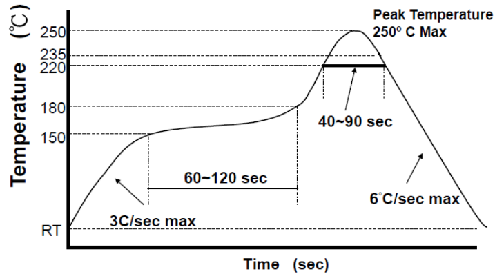
Figure 4-2 Reflow profile
