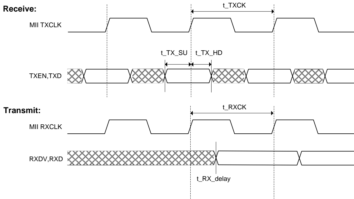
Figure 3-3 RvMII Timing
