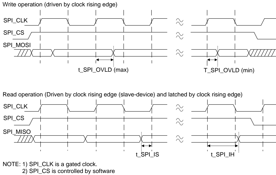
Figure 3-4 SPI Timing
