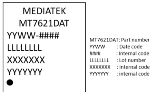
Figure 4-3 Top marking
