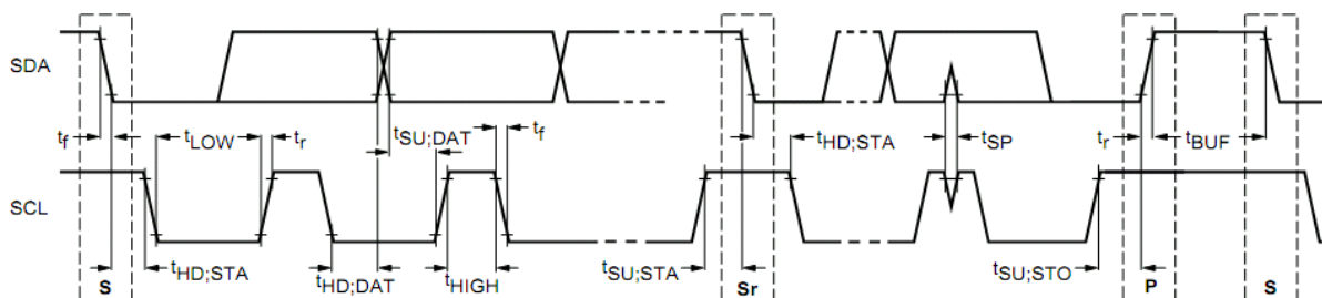
Figure 3-5 I2C Timing
