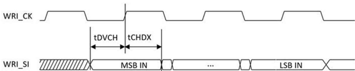
Figure 3-4 WRI Timing
