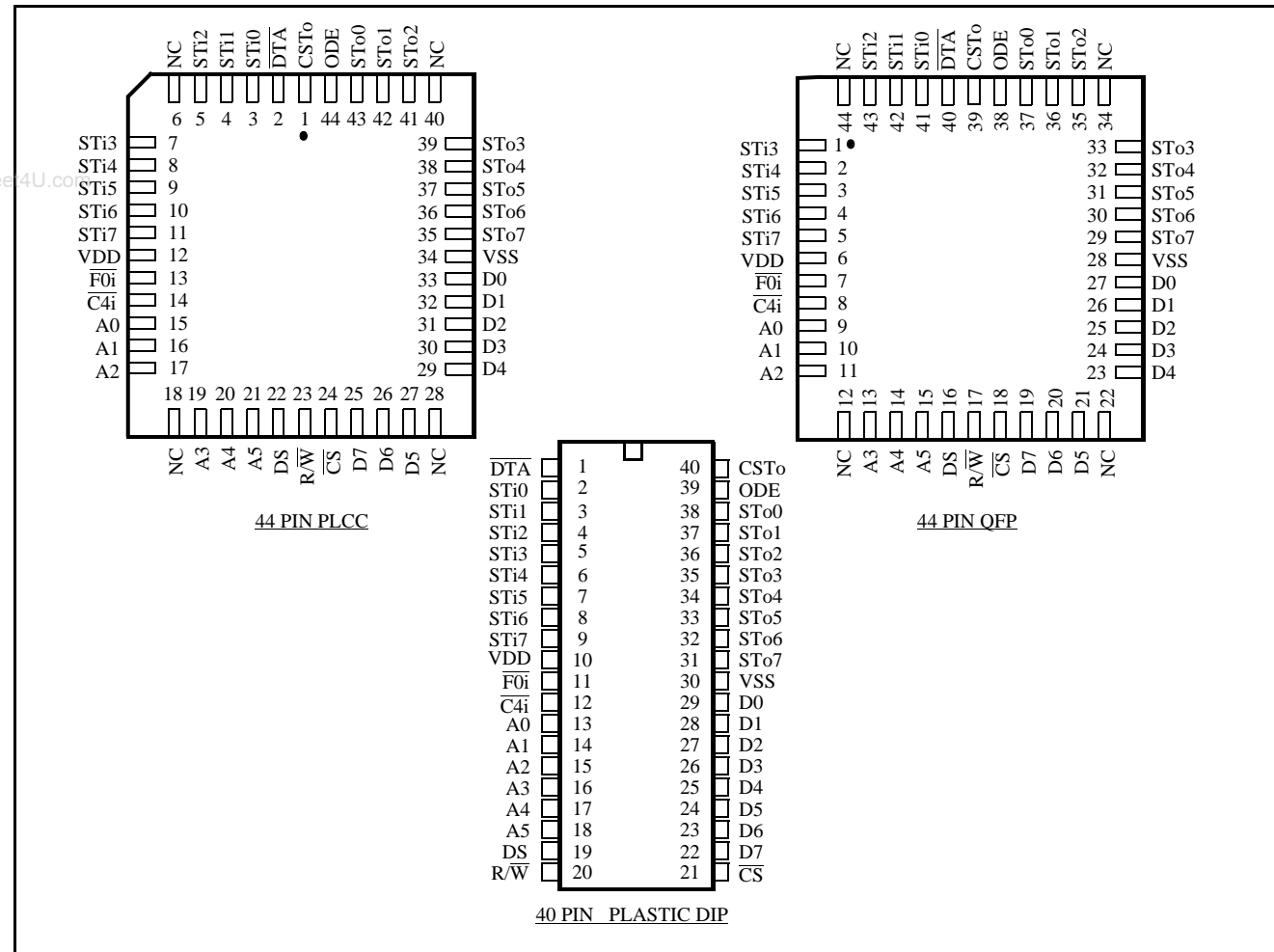
Figure 2 - Pin Connections
